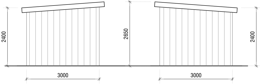
Elevation C SCALE 1:75@A3
