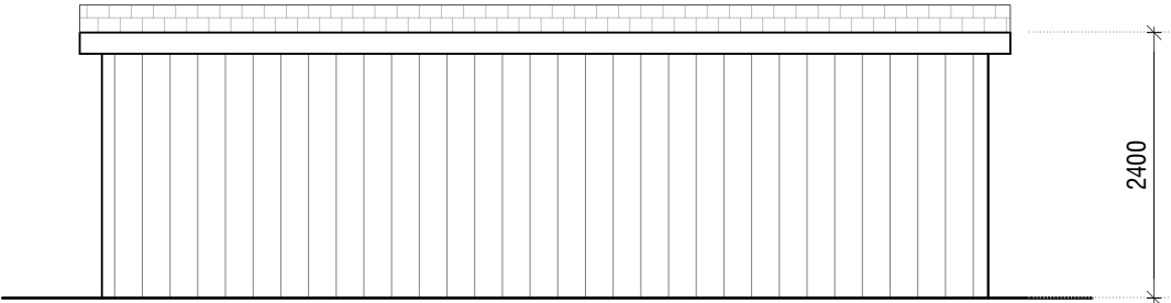
Elevation B SCALE 1:75@A3
