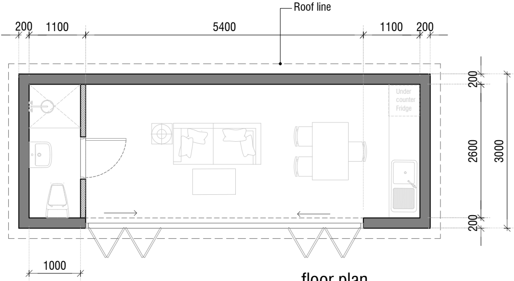
floor plan SCALE 1:75@A3
