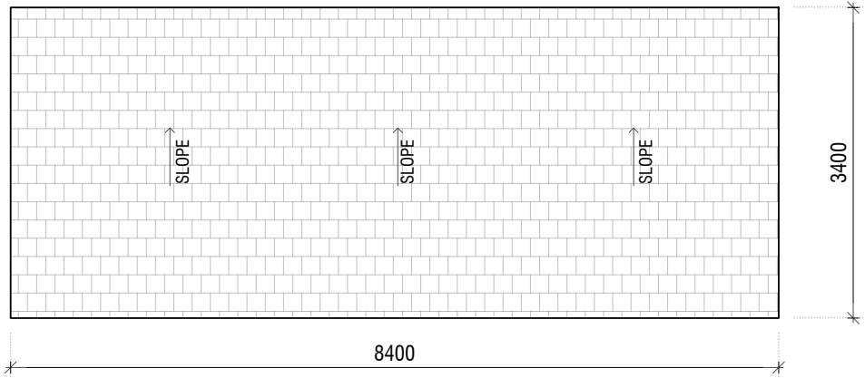
Roof Plan SCALE 1:75@A3
