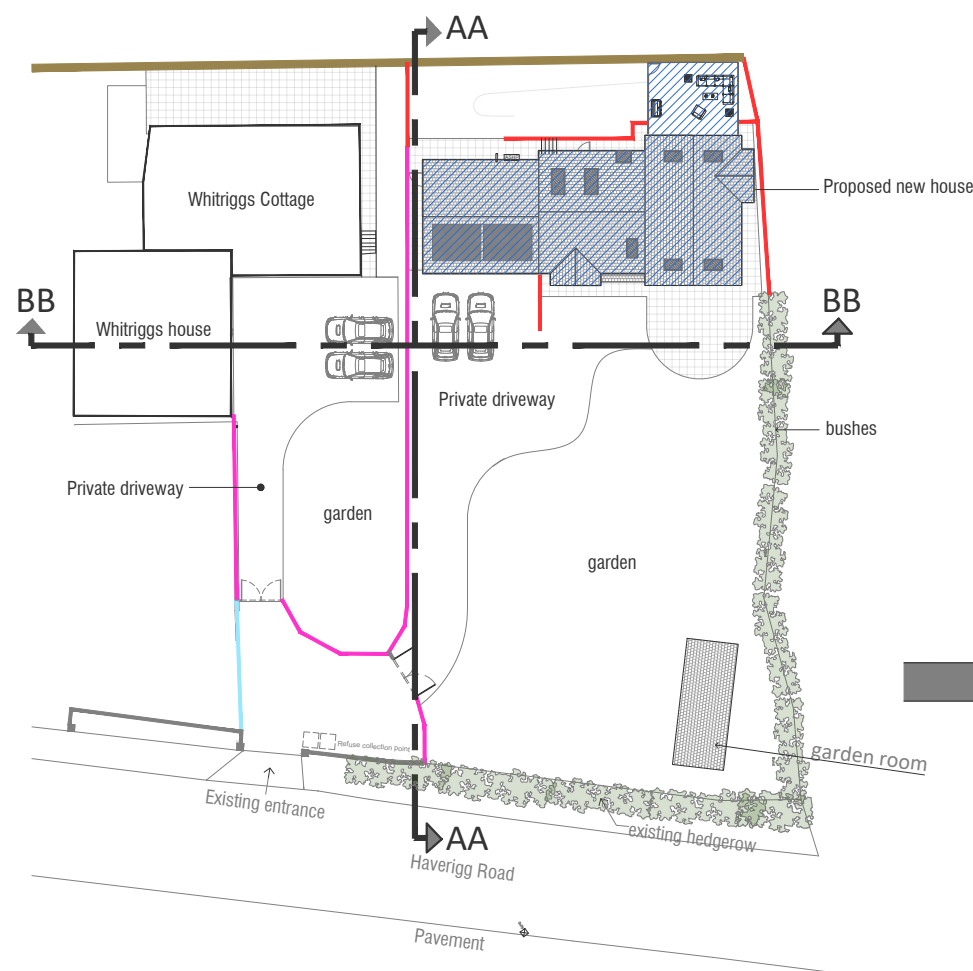
Proposed Site key plan
