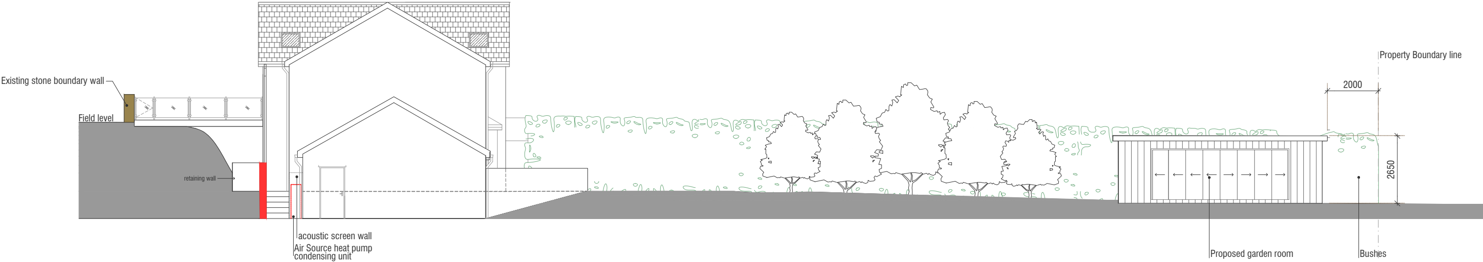
Proposed site section A-A SCALE 1:150@A3
