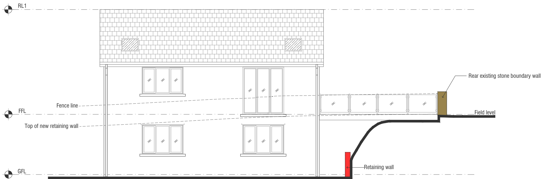
Proposed North East Facing Elevation SCALE 1:100@A3
