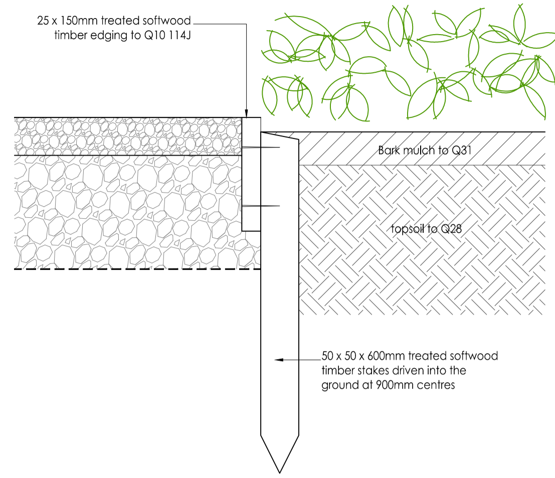
E1a TIMBER EDGE (to tight curves) Scale 1:5. See NBS Q10.114J
