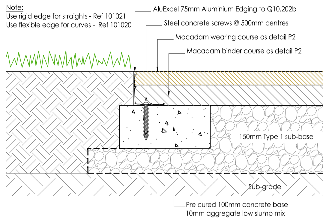
E2b 75mm METAL EDGE (to macadam) Scale 1:5. See NBS Q10.202b
