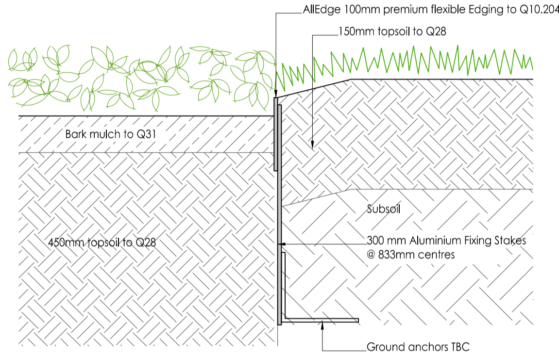
E4 METAL EDGE (to shrub beds / lawn) Scale 1:5. See NBS Q10.204
