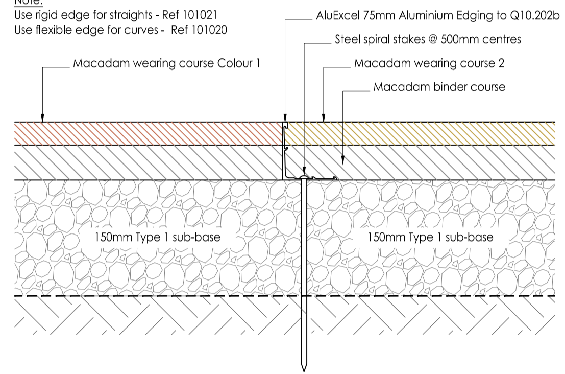
E2b 75mm METAL EDGE (to macadam panel) Scale 1:5. See NBS Q10.202b
