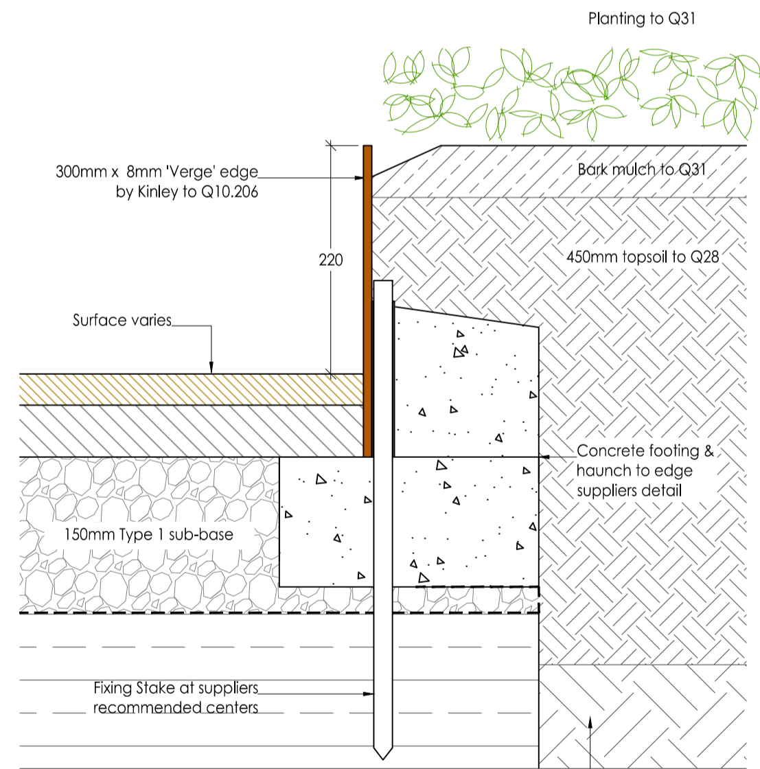
E6 METAL EDGE (200mm Upstand) Scale 1:5. See NBS Q10.206
