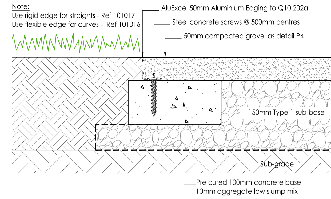
E2a 50mm METAL EDGE (to compacted gravel) Scale 1:5. See NBS Q10.202a
