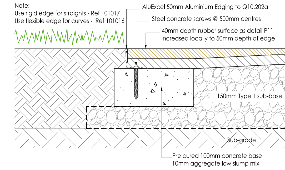
E2a 50mm METAL EDGE (to Rubber Surface) Scale 1:5. See NBS Q10.202a
