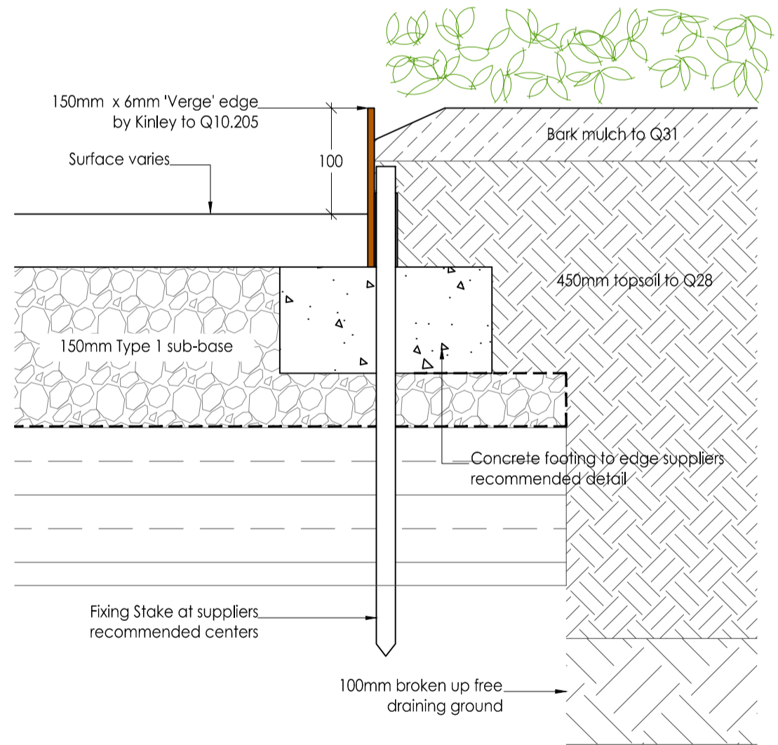
E5 METAL EDGE (100mm upstand) Scale 1:5. See NBS Q10.205
