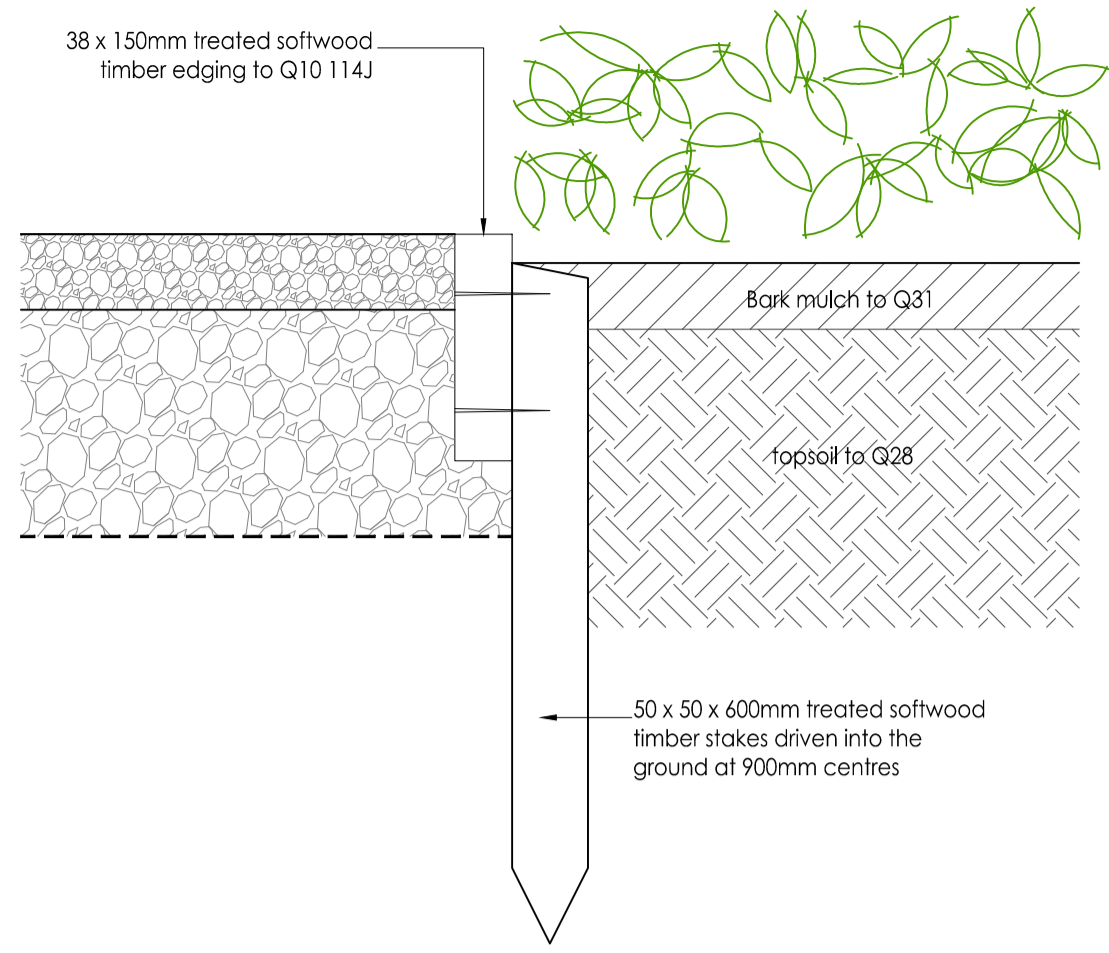
E1 TIMBER EDGE (to straights & gentle curves) Scale 1:5. See NBS Q10.114J
