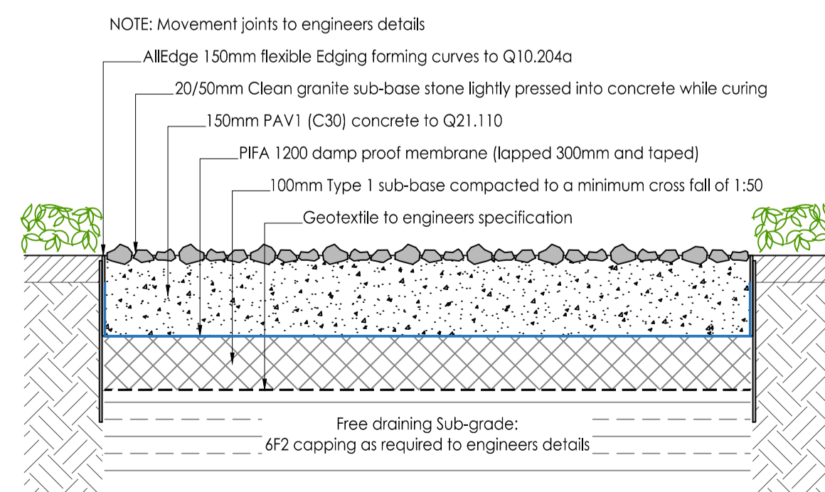
SP1 MIXED REHABILITATION CHALLENGE PAVING - GRAVEL A Scale 1:10. See NBS Q25.165J
