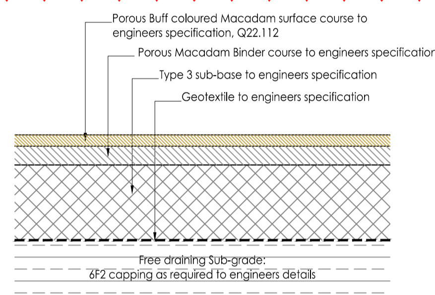
P2a BUFF MACADAM (COURTYARD) 0101 Scale 1:10. See NBS Q22.112 (Permeable to courtyard only)
