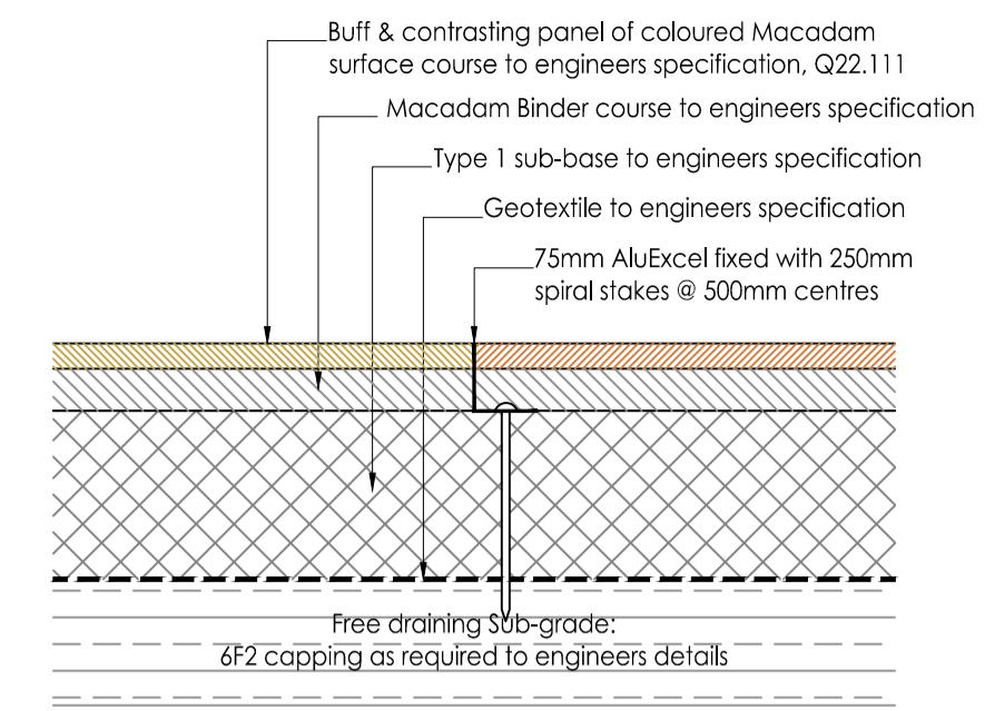
P2 BUFF & COLOURED MACADAM (PEDESTRIAN) 0101 Scale 1:10. See NBS Q22.111 (non permeable)
