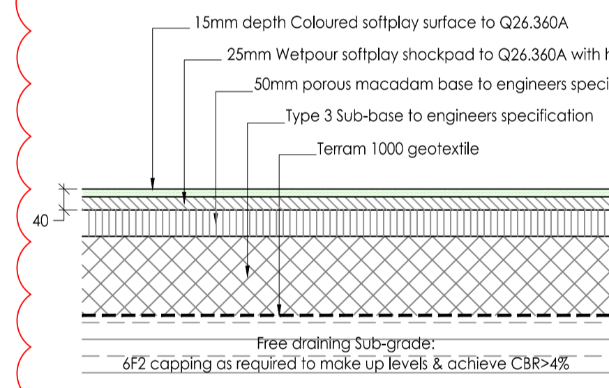
P11 PERMEABLE SOFT PLAY RUBBER SURFACING 0101 Scale 1:10. See NBS Q26.360A
