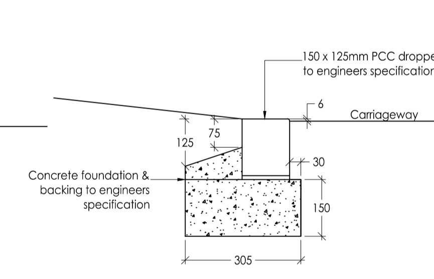
K3 PCC DROPPED ROAD KERB (6mm) 0101 Scale 1:10. See NBS Q10.110J
