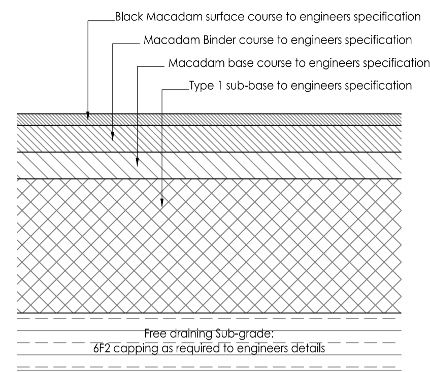
P1b BLACK MACADAM (VEHICULAR) 0101 Scale 1:10. See NBS Q22.107J
