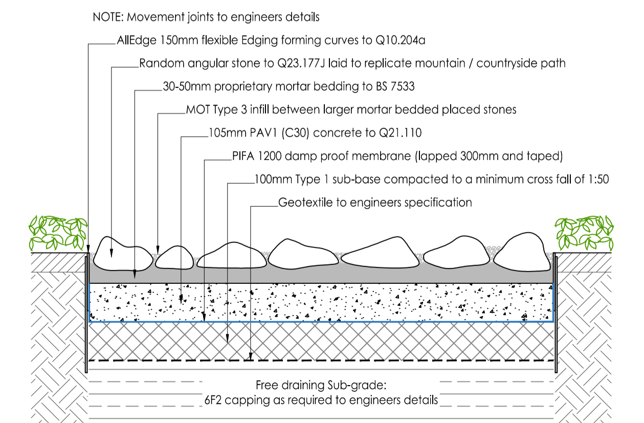
SP1 MIXED REHABILITATION CHALLENGE PAVING - ANGULAR STONE D Scale 1:10. See NBS Q25.165J
