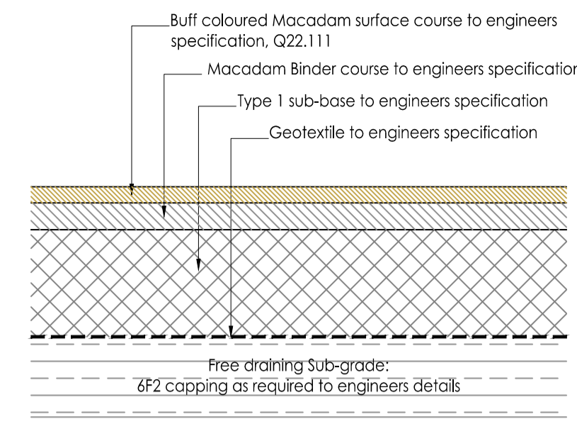
P2 BUFF MACADAM (PEDESTRIAN) 0101 Scale 1:10. See NBS Q22.111 (non permeable)
