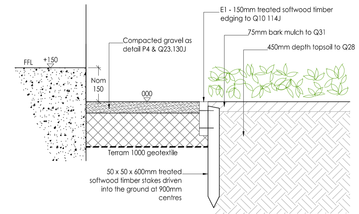
P4a SELF BINDING GRAVEL EDGE TO BUILDING 0101 Scale 1:10. See NBS Q23.130J
