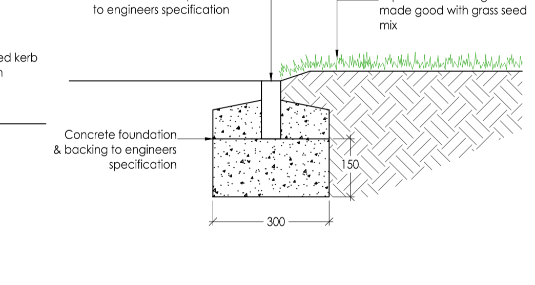
K4 PCC PIN KERB (Flush) 0101 Scale 1:10. See NBS Q10.112
