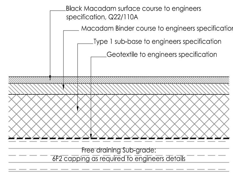
P1 BLACK MACADAM (PEDESTRIAN) 0101 Scale 1:10. See NBS Q22.110A
