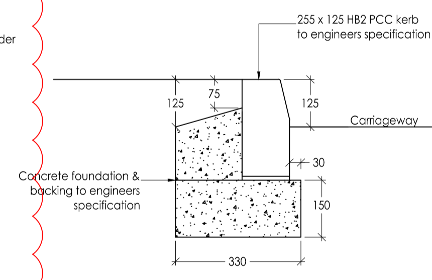
K1 PCC ROAD KERB 0101 Scale 1:10. See NBS Q10.110J
