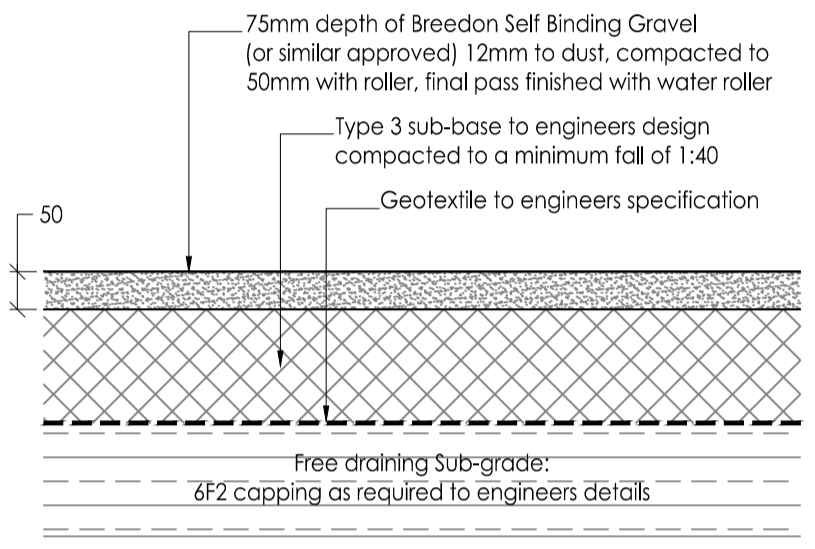
P4 SELF BINDING GRAVEL 0101 Scale 1:10. See NBS Q23.130J
