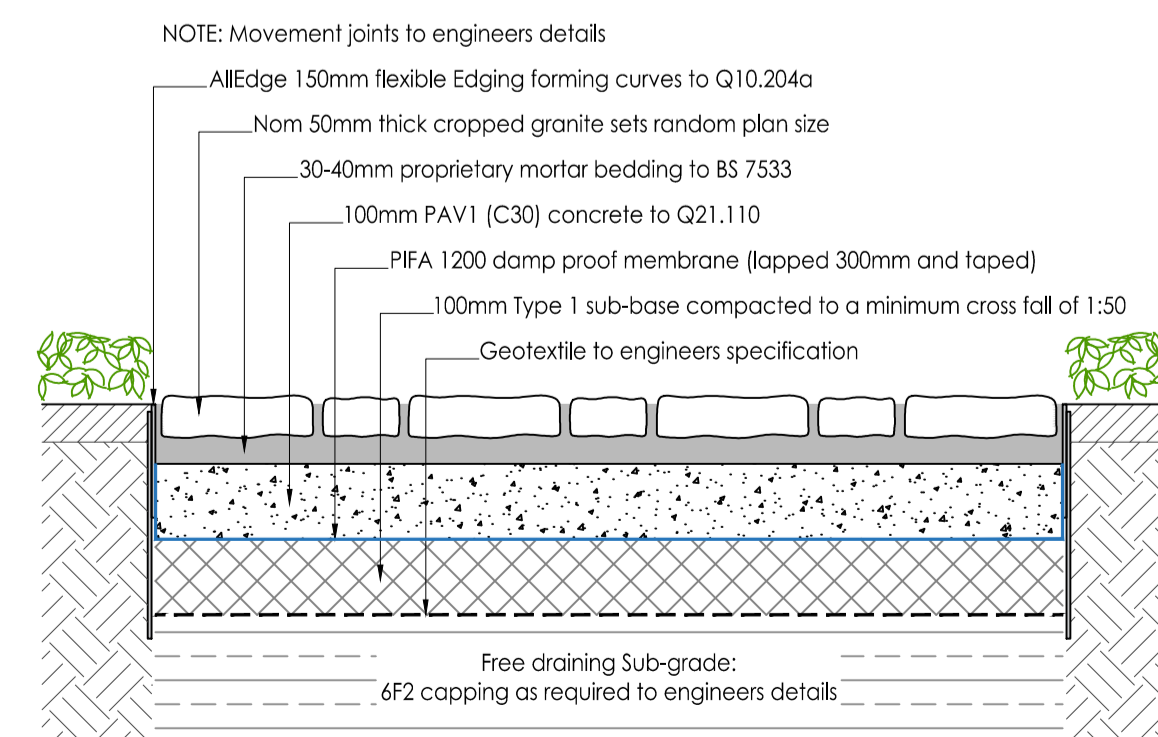
SP1 MIXED REHABILITATION CHALLENGE PAVING - CROPPED SETTS B Scale 1:10. See NBS Q25.165J
