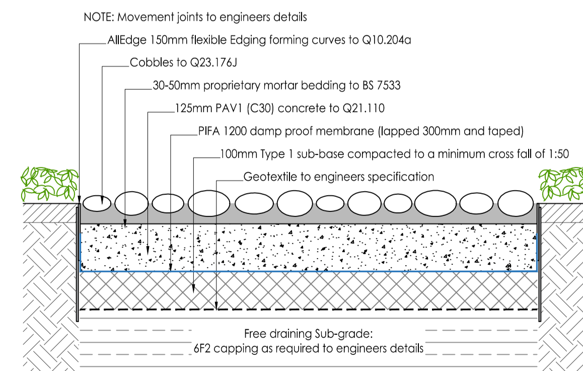
SP1 MIXED REHABILITATION CHALLENGE PAVING - COBBLES C Scale 1:10. See NBS Q25.165J
