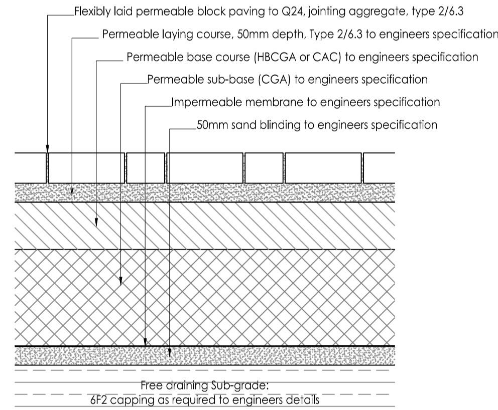
P06 PERMEABLE FLEXIBLE BLOCK PAVING (VEHICULAR) 0101 Scale 1:10. See NBS Q24.115
