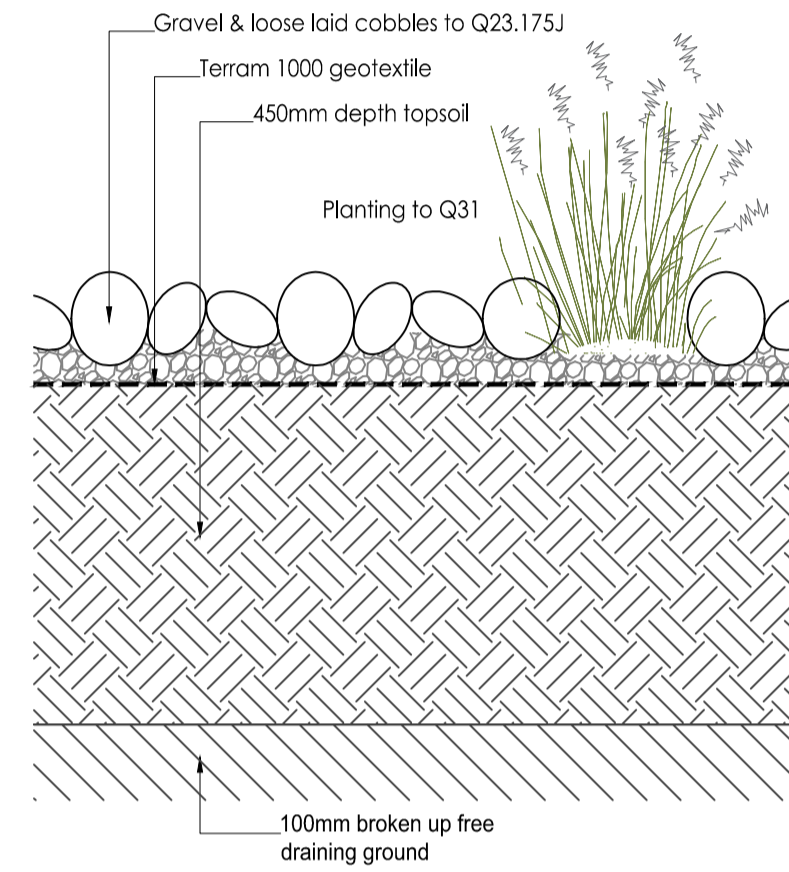
P3 COBBLES & BOULDERS 0101 Scale 1:10. See NBS Q23.175J
