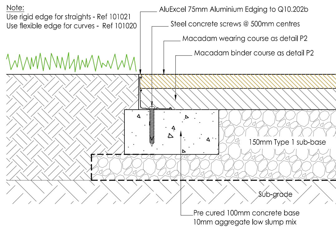
E2b 75mm METAL EDGE (to macadam) 0100 Scale 1:5. See NBS Q10.202b
