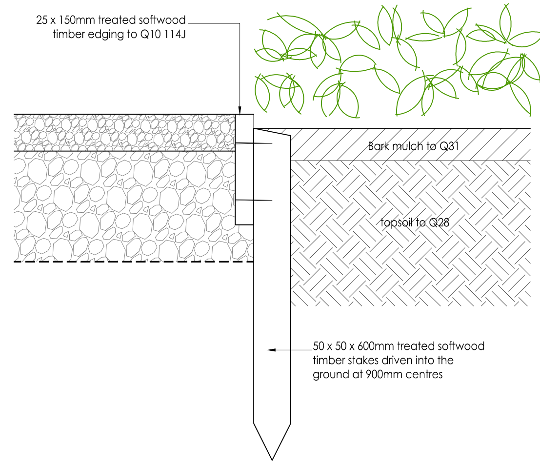
E1a TIMBER EDGE (to tight curves) 0100 Scale 1:5. See NBS Q10.114J
