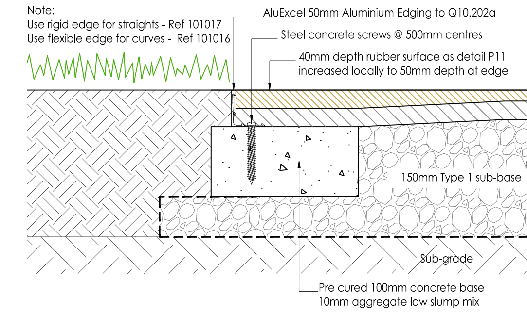
E2a 50mm METAL EDGE (to Rubber Surface) 0100 Scale 1:5. See NBS Q10.202a
