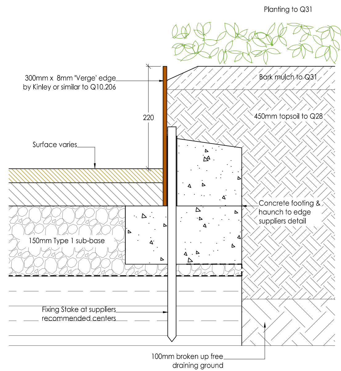
E6 METAL EDGE (200mm Upstand) 0100 Scale 1:5. See NBS Q10.206
