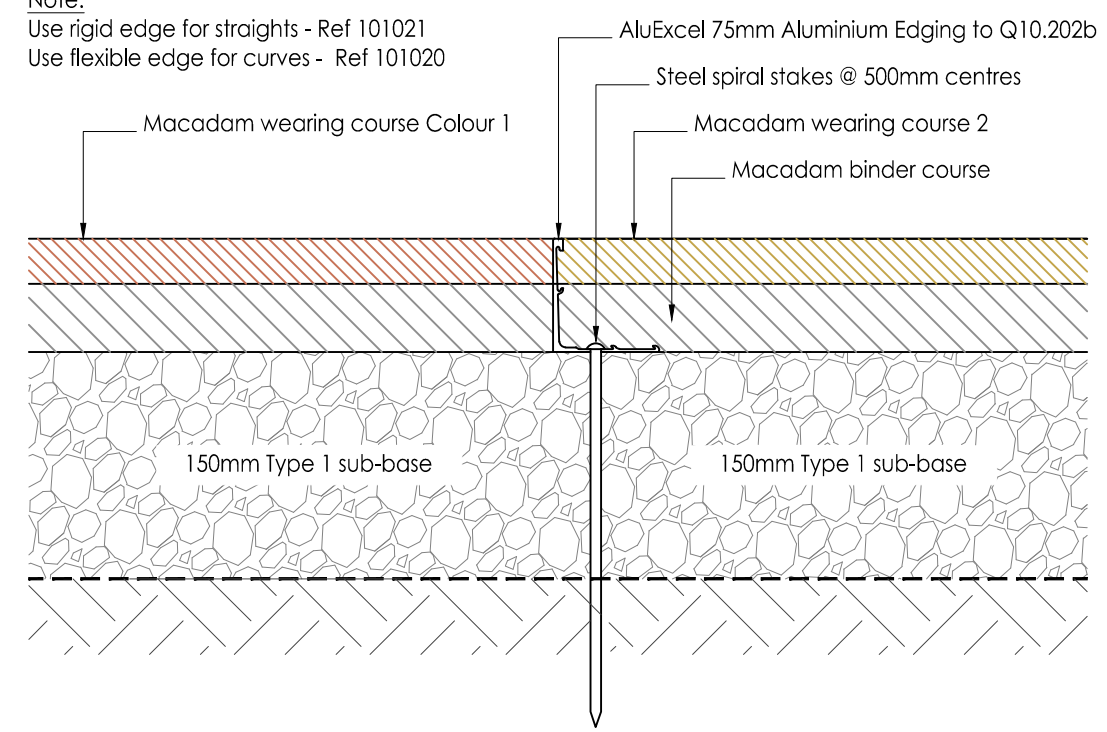
E2b 75mm METAL EDGE (to macadam panel) 0100 Scale 1:5. See NBS Q10.202b
