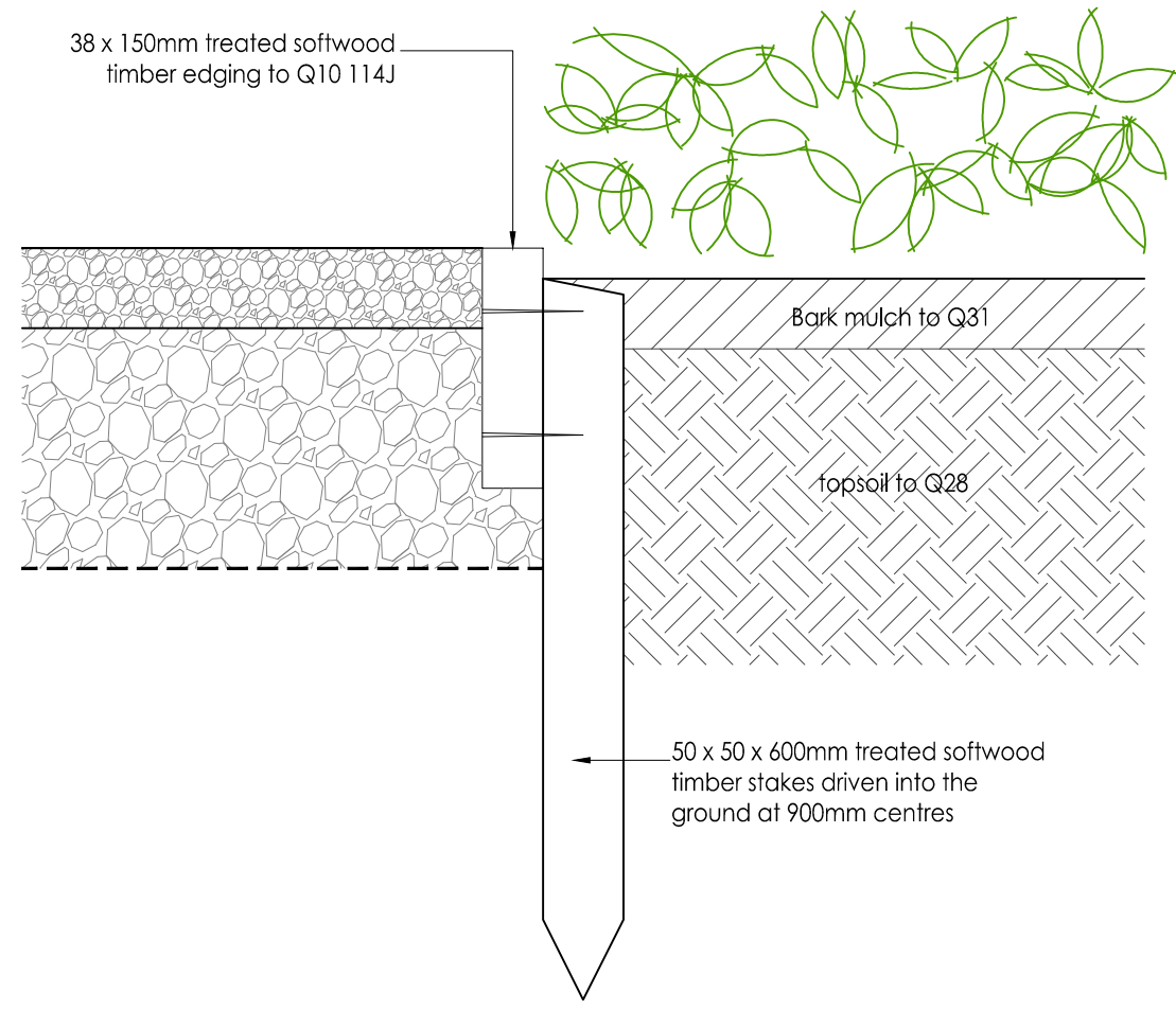
E1 TIMBER EDGE (to straights & gentle curves) 0100 Scale 1:5. See NBS Q10.114J
