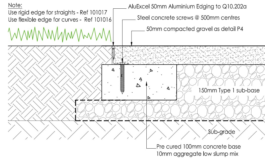
E2a 50mm METAL EDGE (to compacted gravel) 0100 Scale 1:5. See NBS Q10.202a
