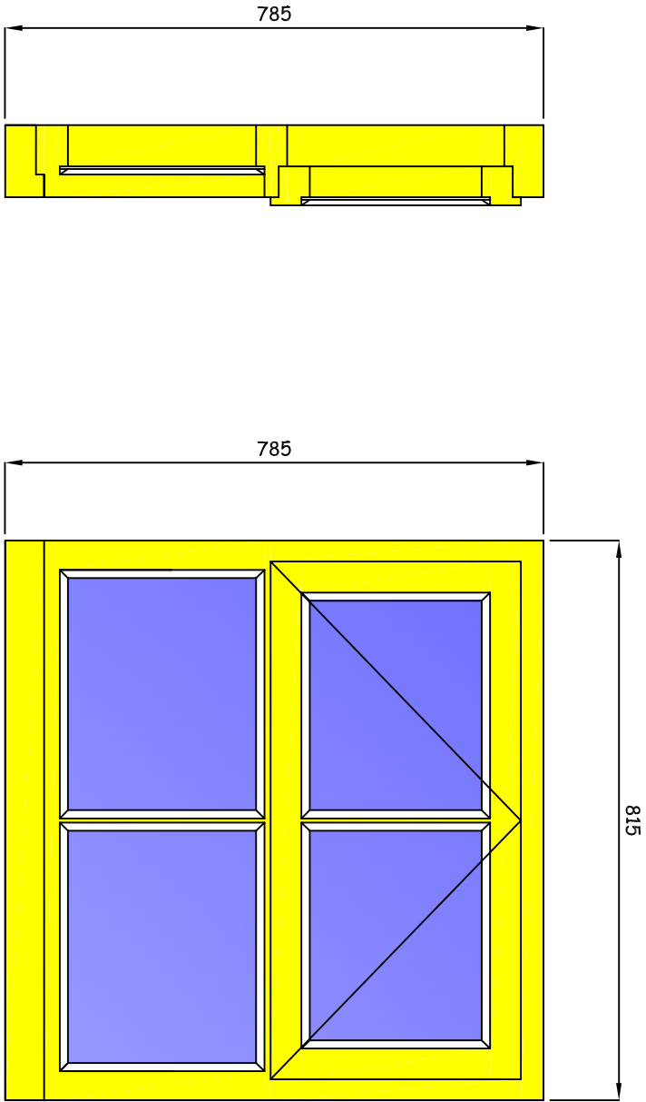
Section through window
