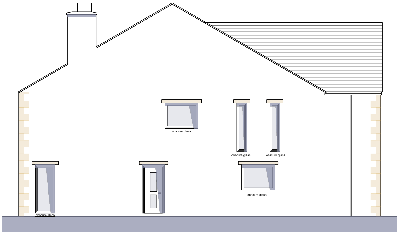
SIDE ELEVATION
