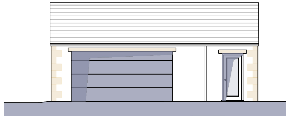
2 Garage Front Elevation 1:100
