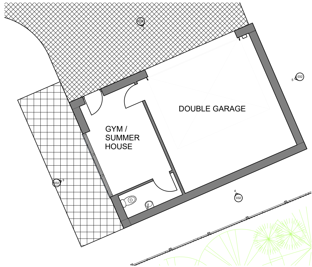
1 Plot 3 Garage Plan 1:100
