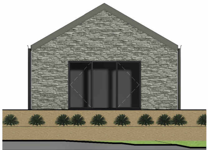
3 Garage Side Elevation 1 : 100
