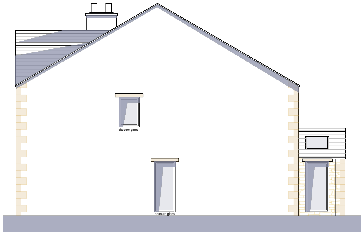
SIDE ELEVATION
