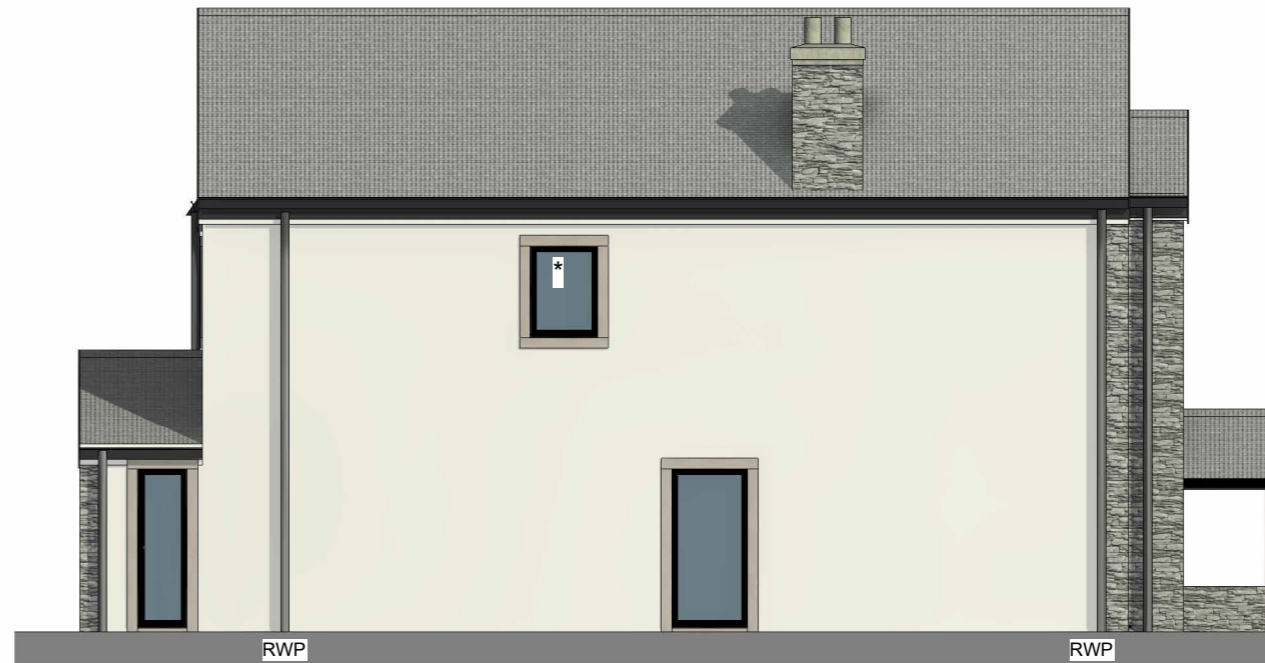
4 West Elevation 1 : 100
