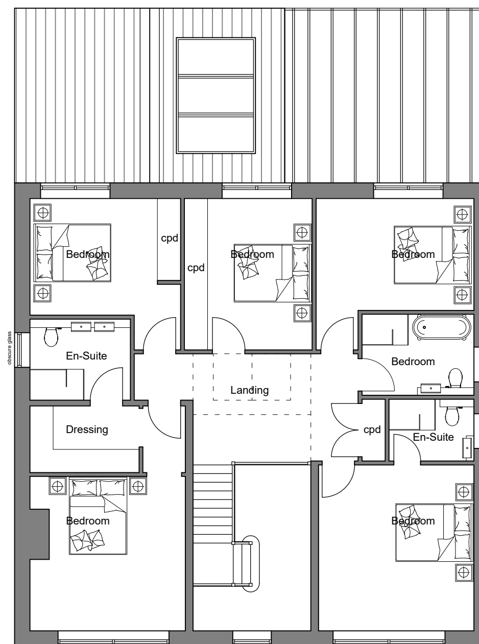
FIRST FLOOR
