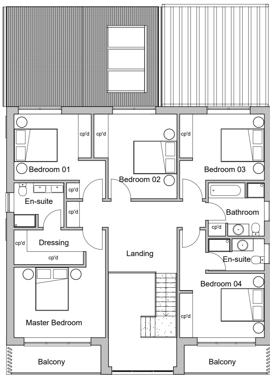
2 First Floor Plan 1 : 100
