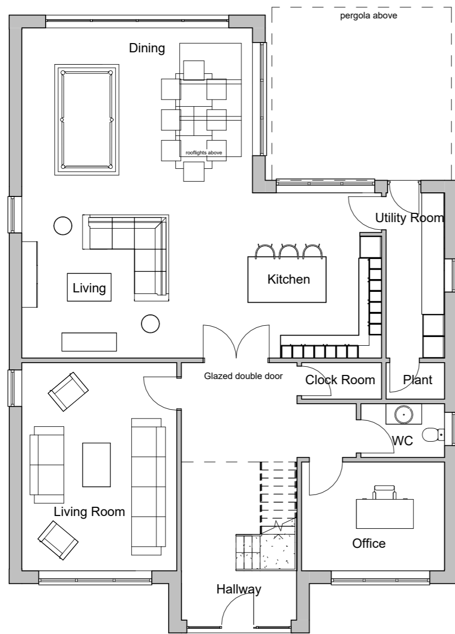
1 Ground Floor Plan 1 : 100
