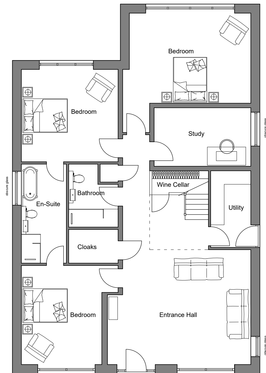
GROUND FLOOR
