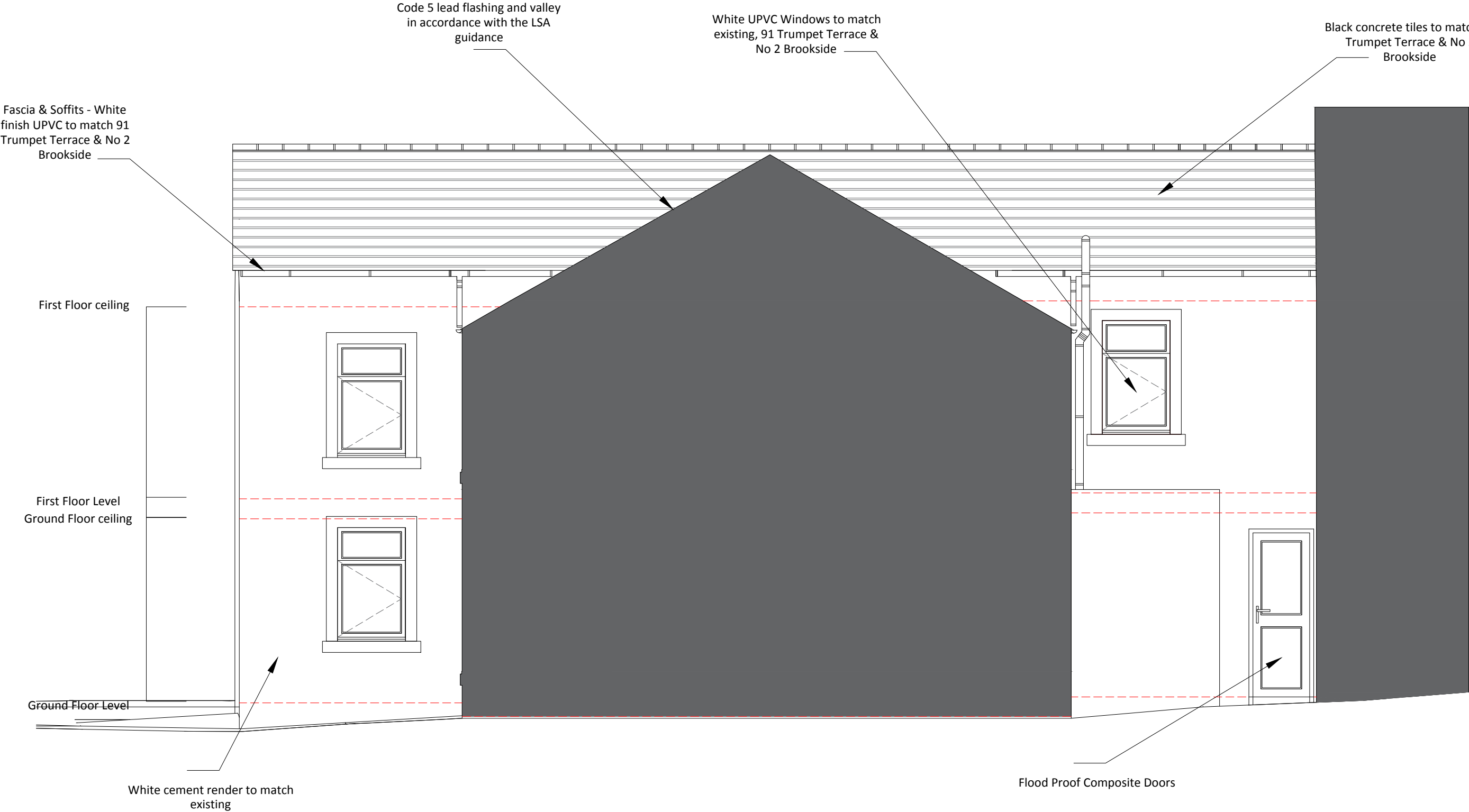
South Elevation
