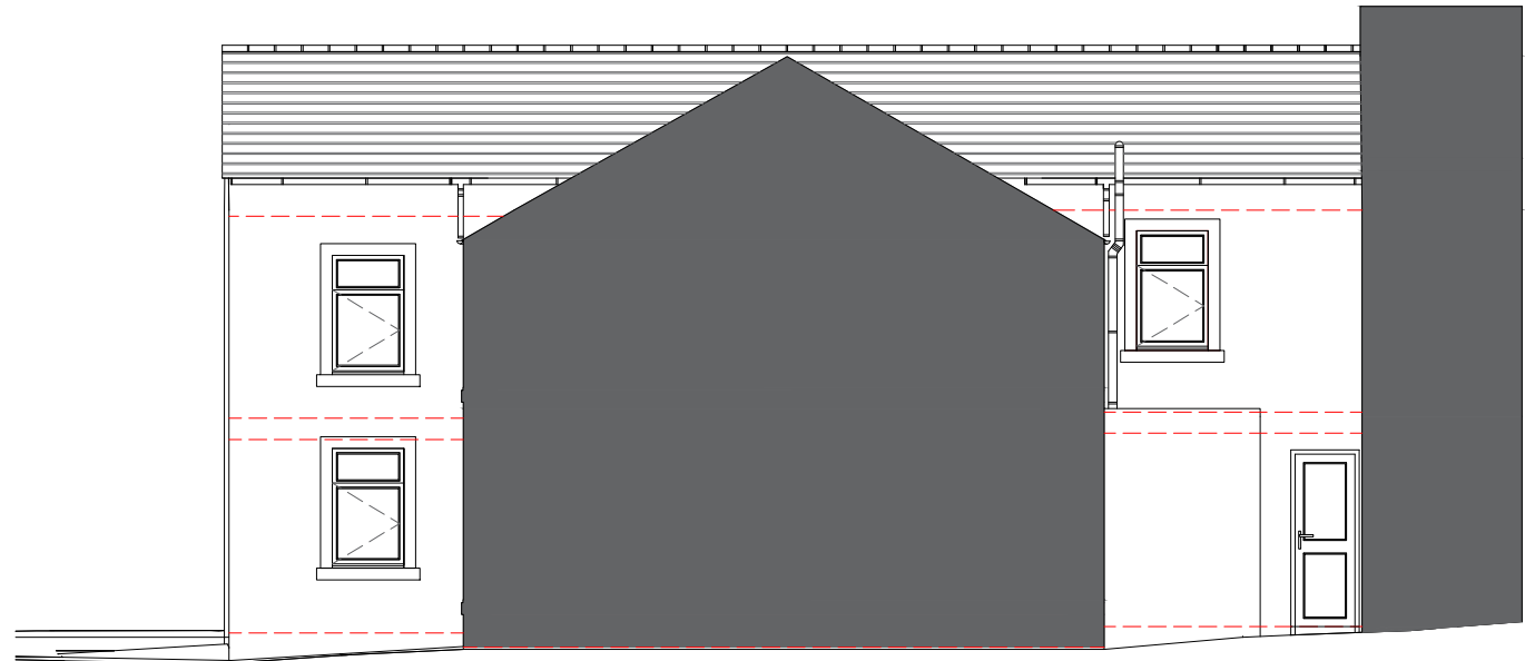
South Elevation
