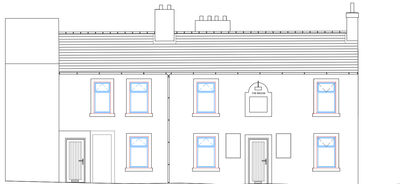
North Elevation
