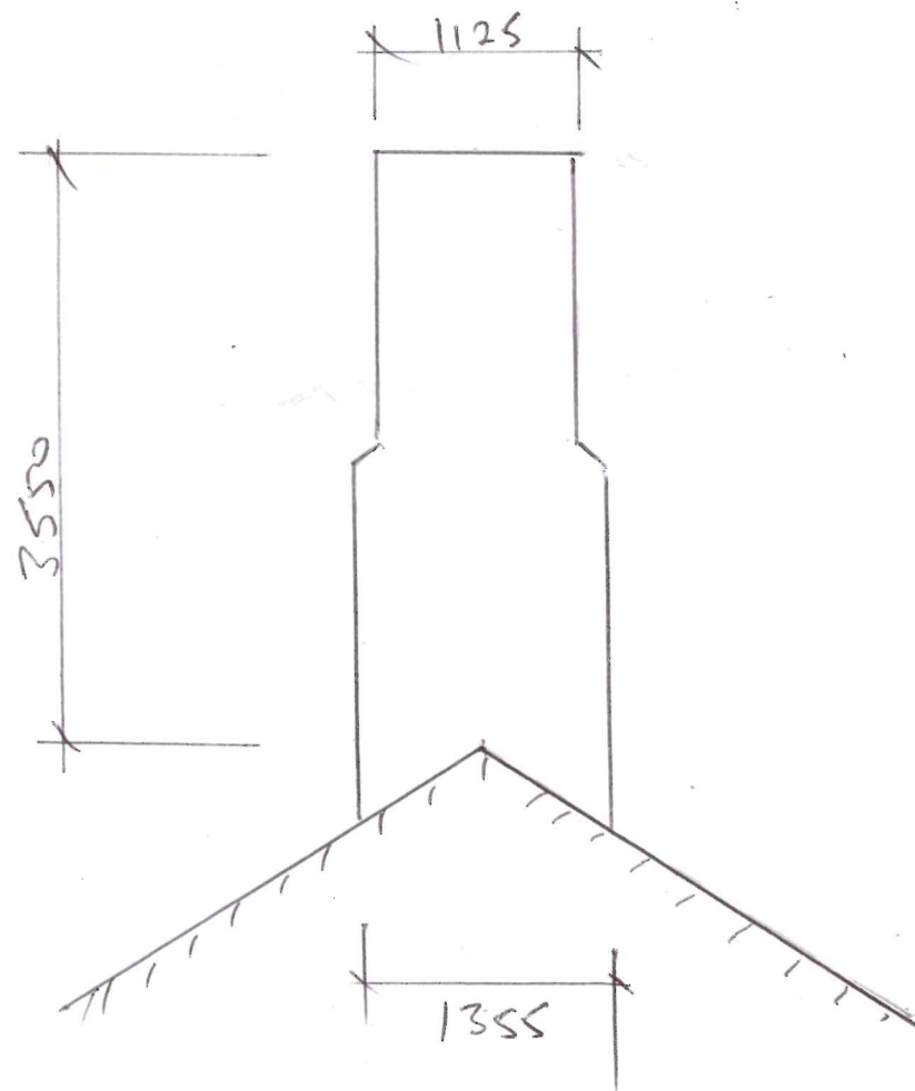
EXISTING STACK (ELEVATION)
