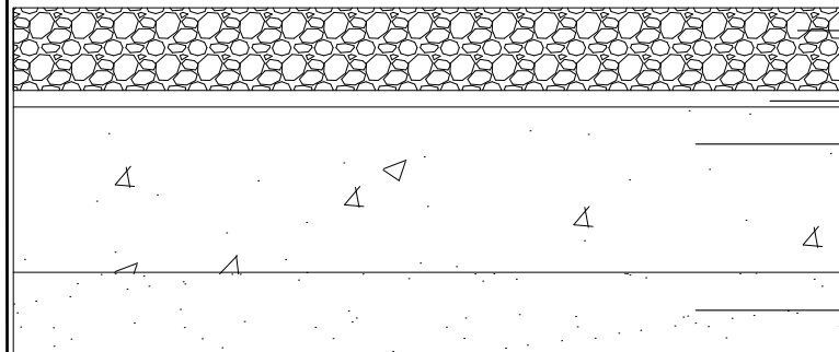
SUDS TRACK SECTION SCALE 1:5
