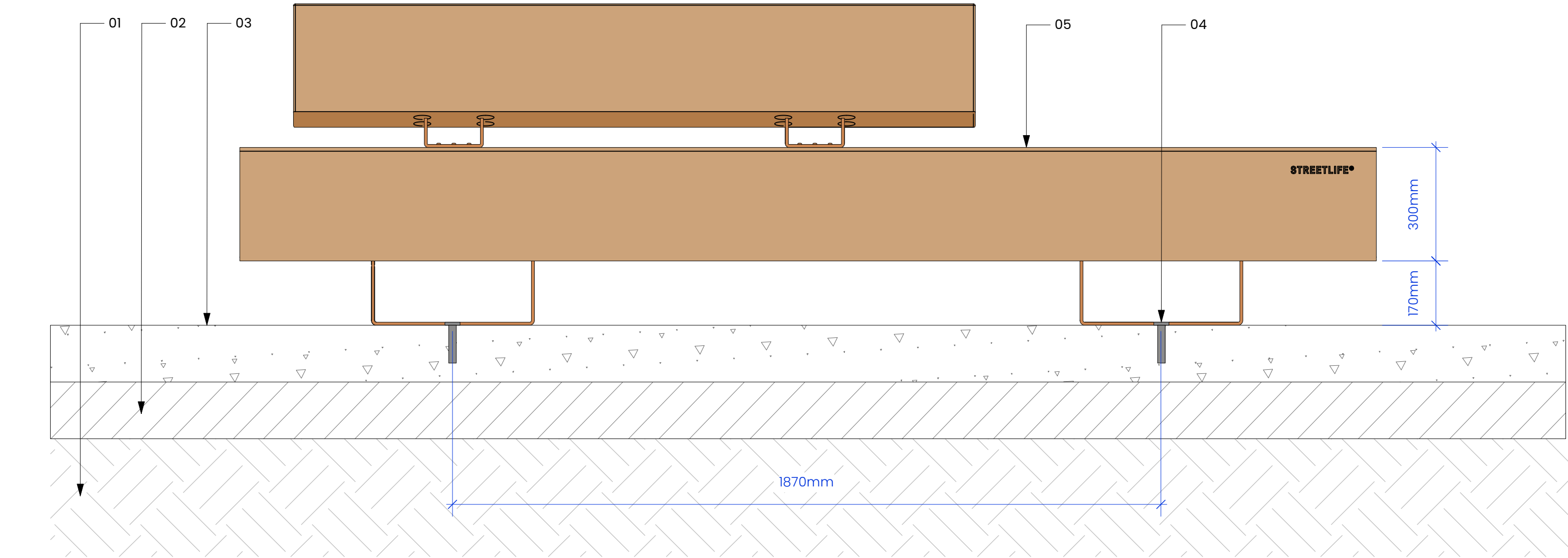
D01 Streetlife Bench Detail Scale: 1:10
