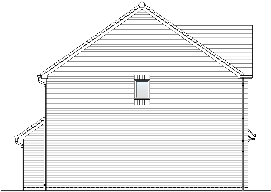
Left Elevation
