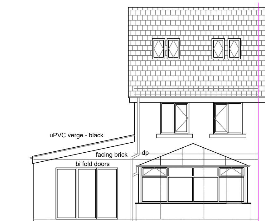
Rear Elevation
