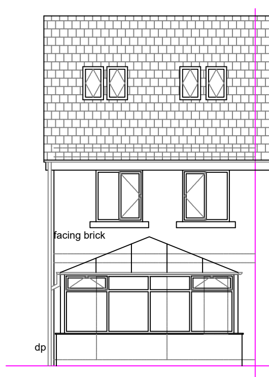
Rear Elevation
