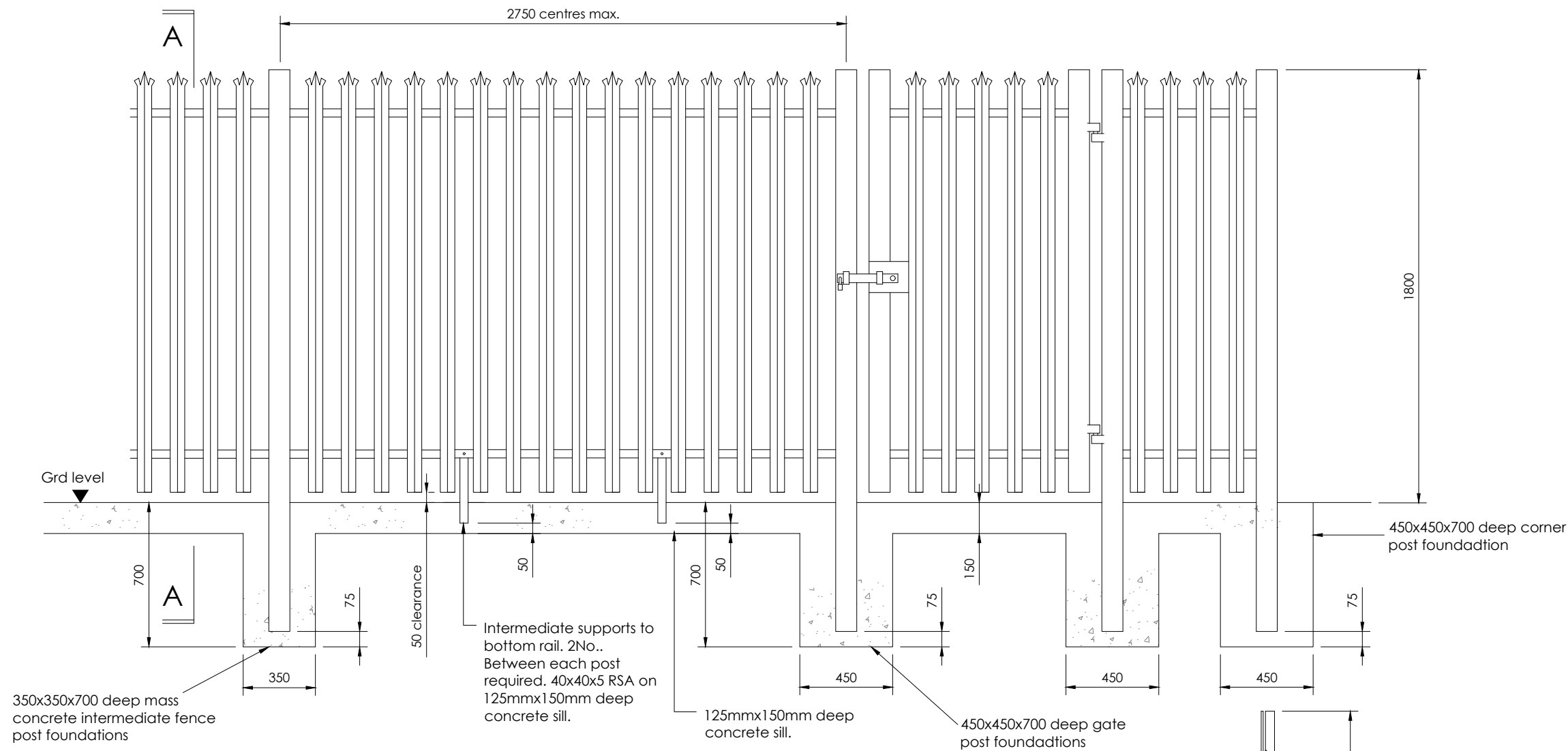
PALISADE FENCE ELEVATION Scale 1:25
