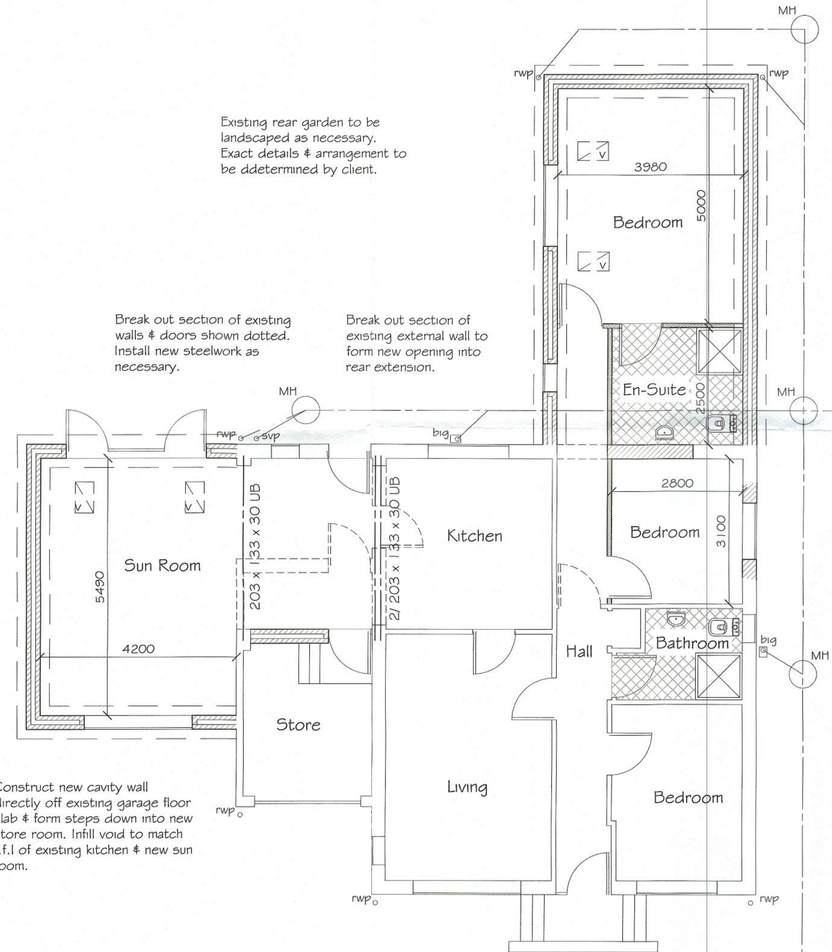
GROUND FLOOR PLAN AS PROPOSED Scale 1:50
