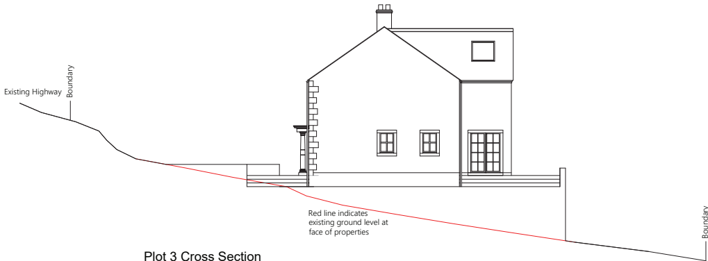
Plot 3 Cross Section
