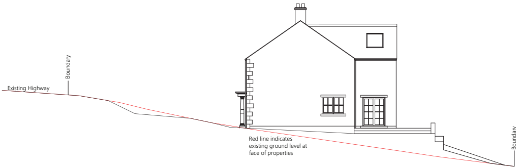
Plot 2 Cross Section
