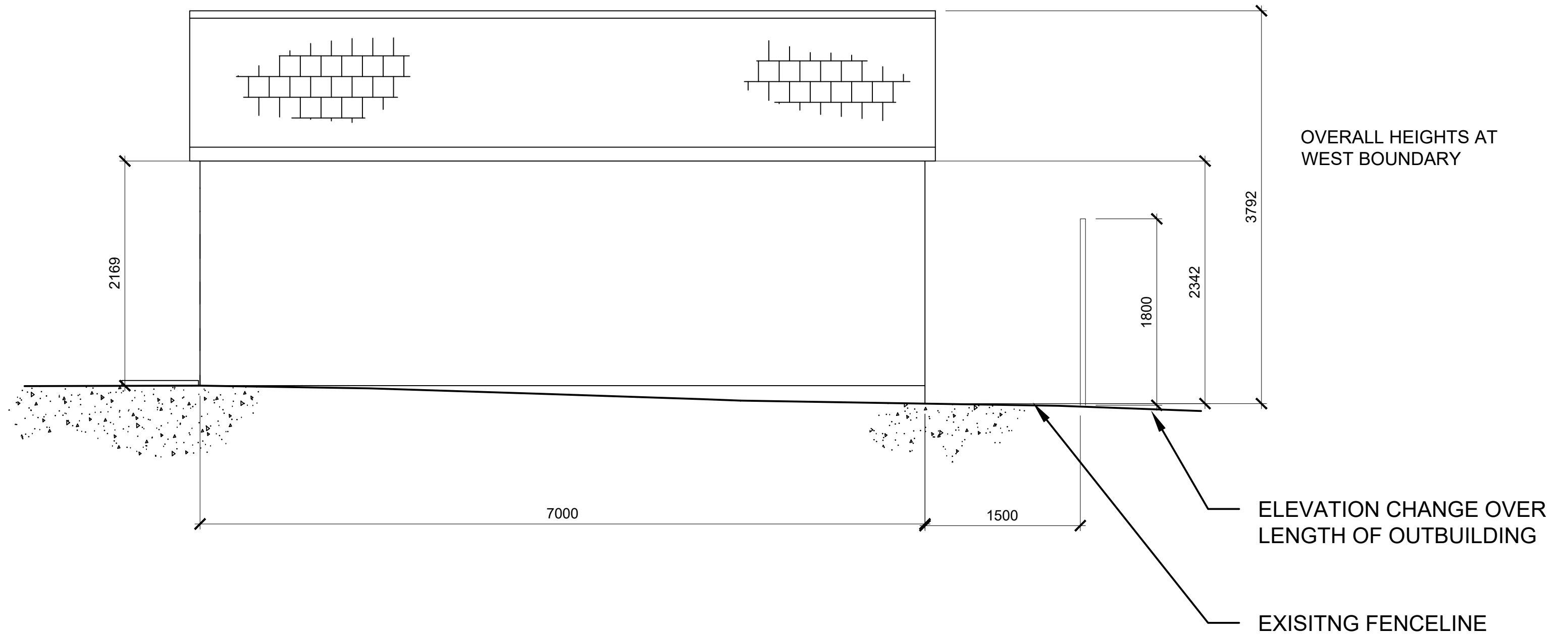
SIDE ELEVATION VIEW LOOKING SOUTH SES Rev B
