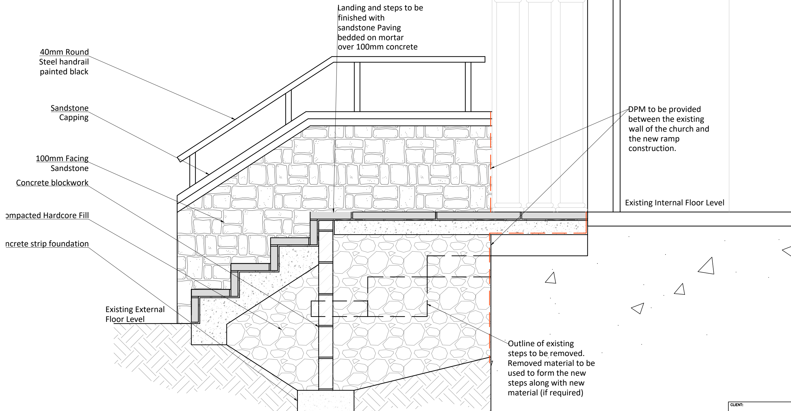
Section Showing Interface with Existing Entrance
