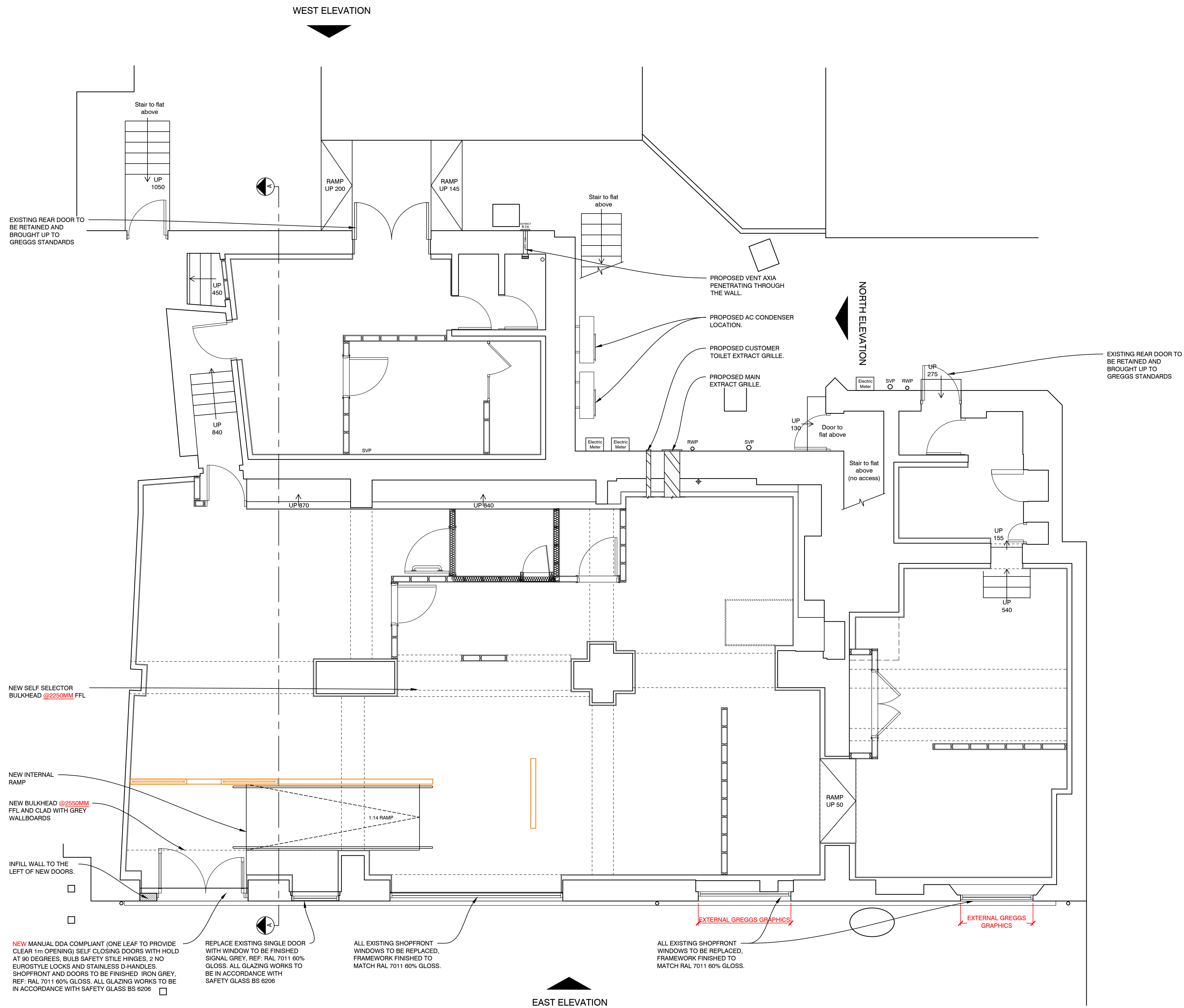
PROPOSED GA PLAN (1:50)
