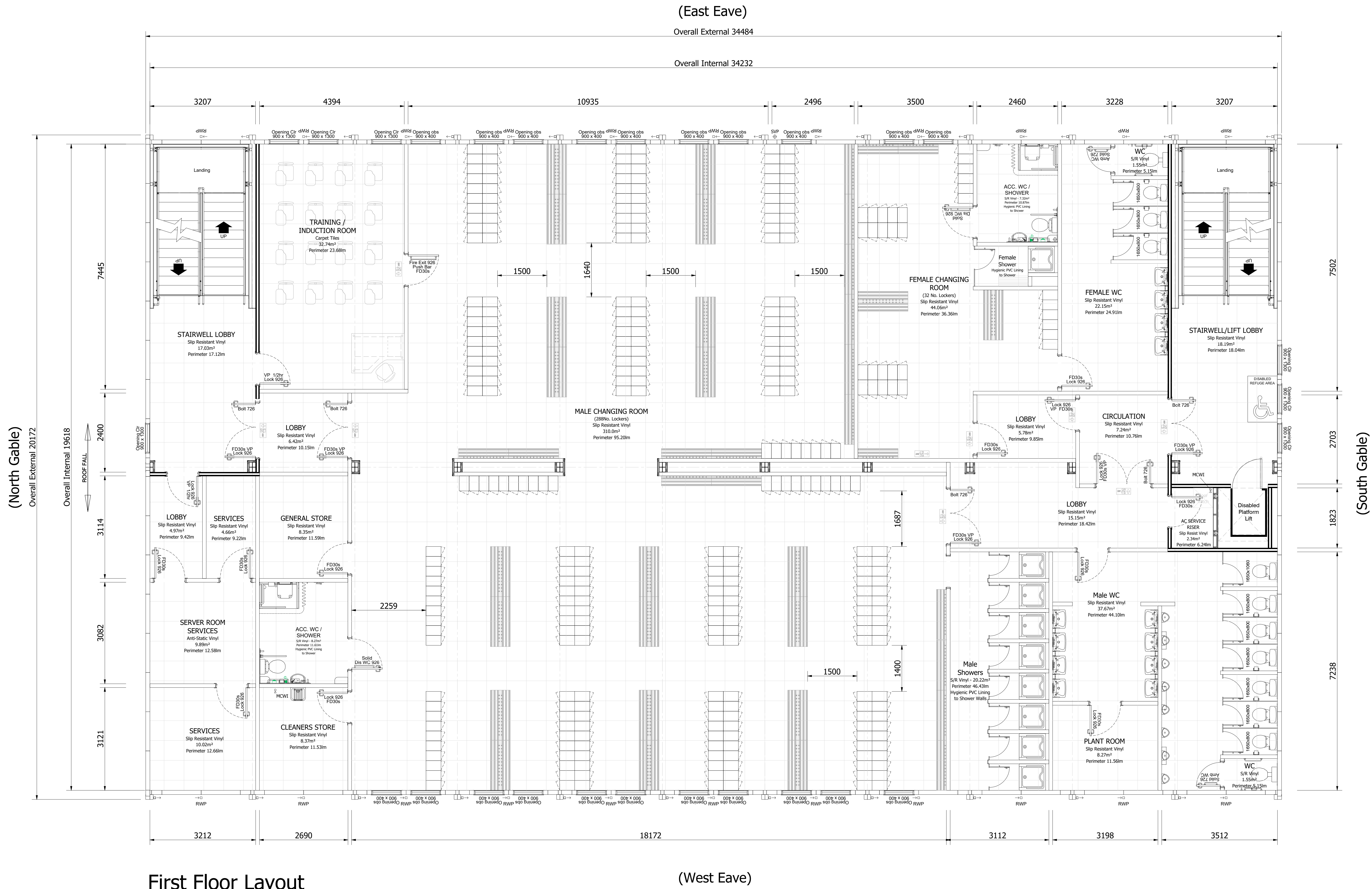
First Floor Layout
