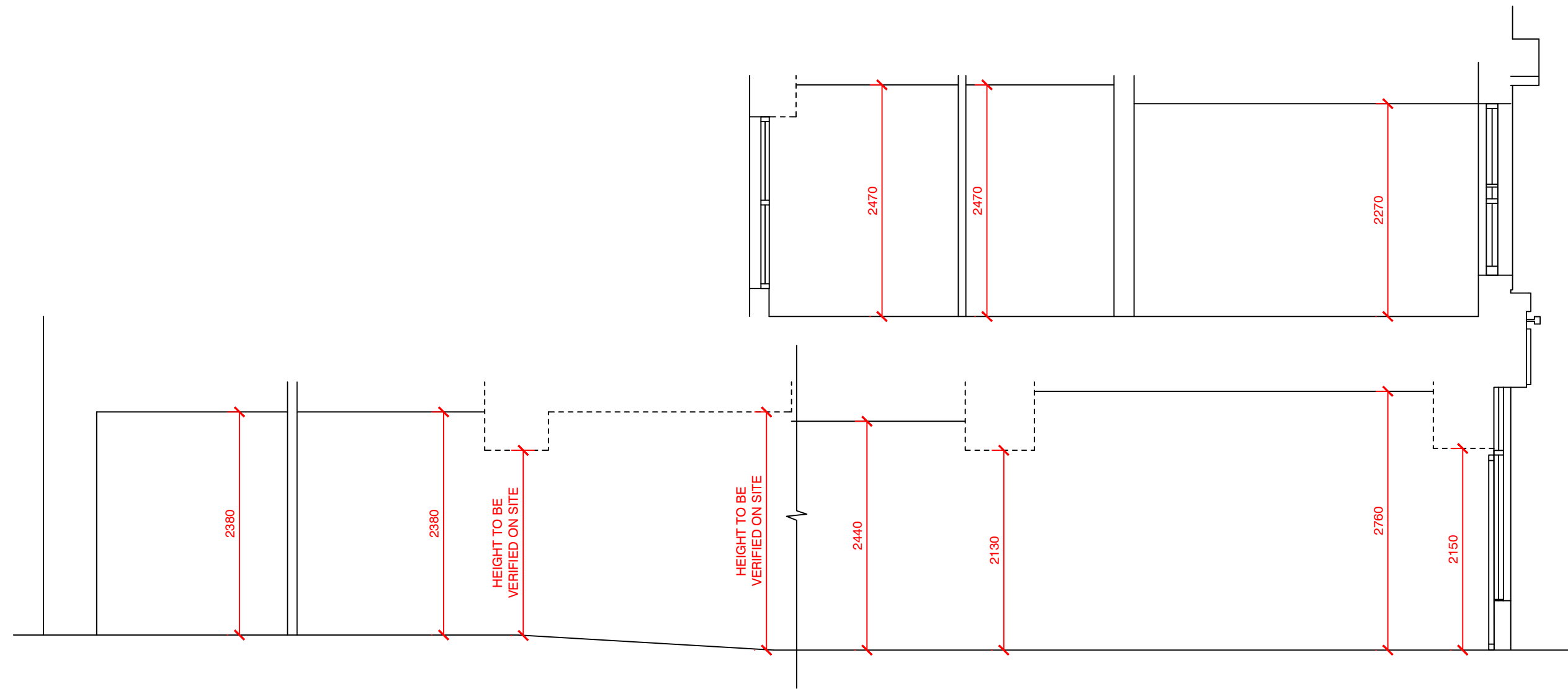
EXISTING SECTION C-C (1:50)
