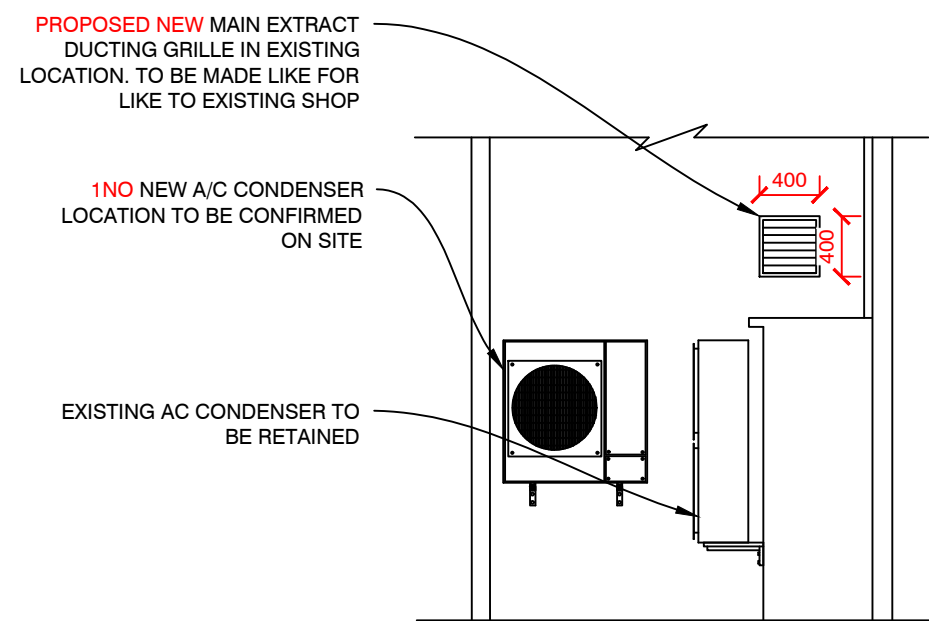
PROPOSED SECTION F-F (1:50)
