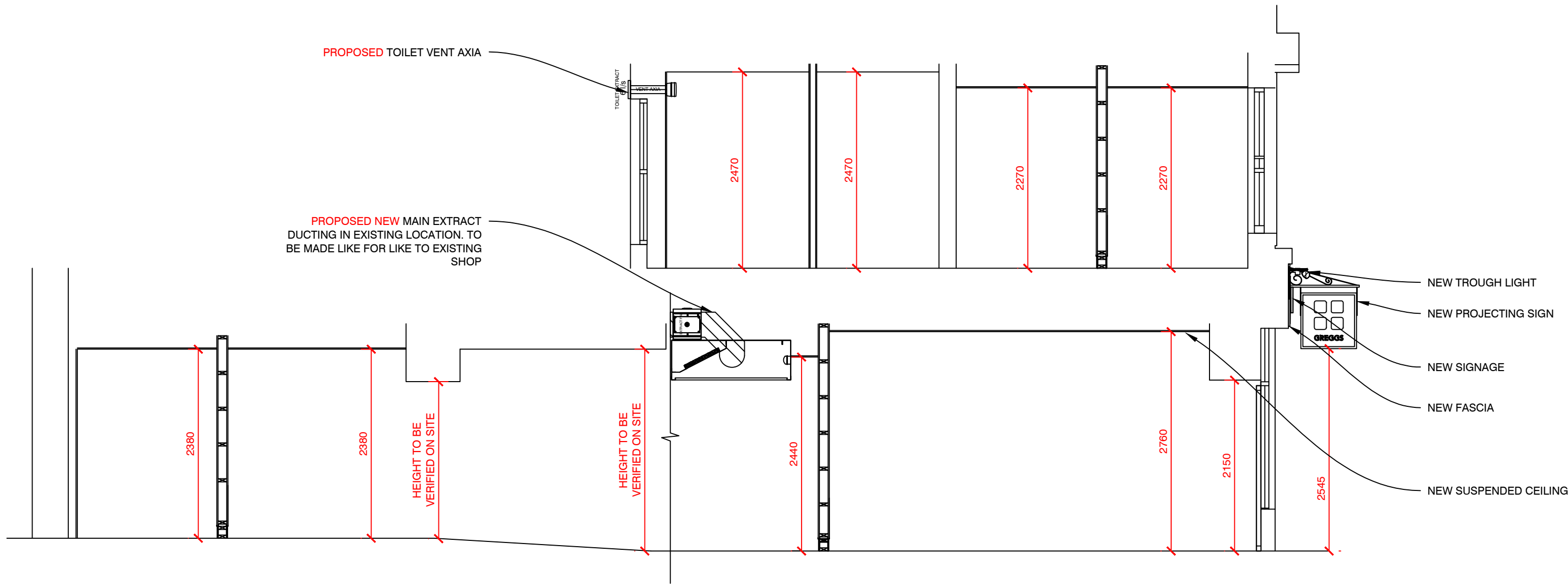
PROPOSED SECTION C-C (1:50)
