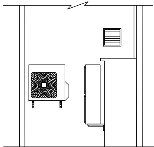
EXISTING SECTION F-F (1:50)
