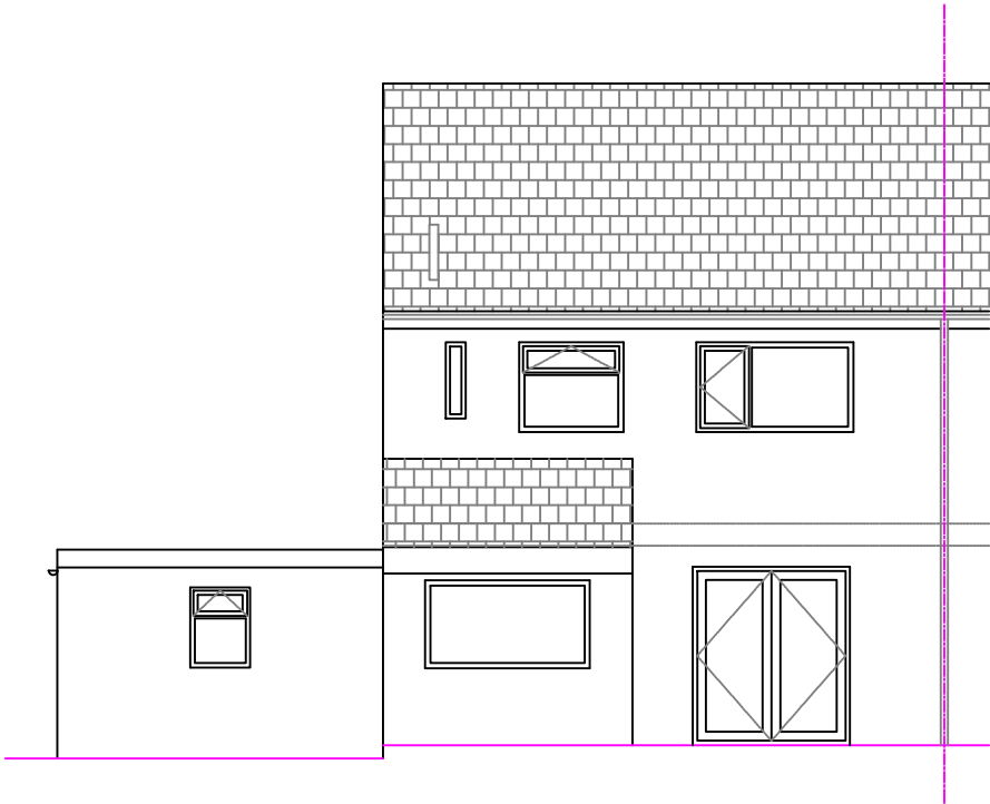
Rear Elevation
