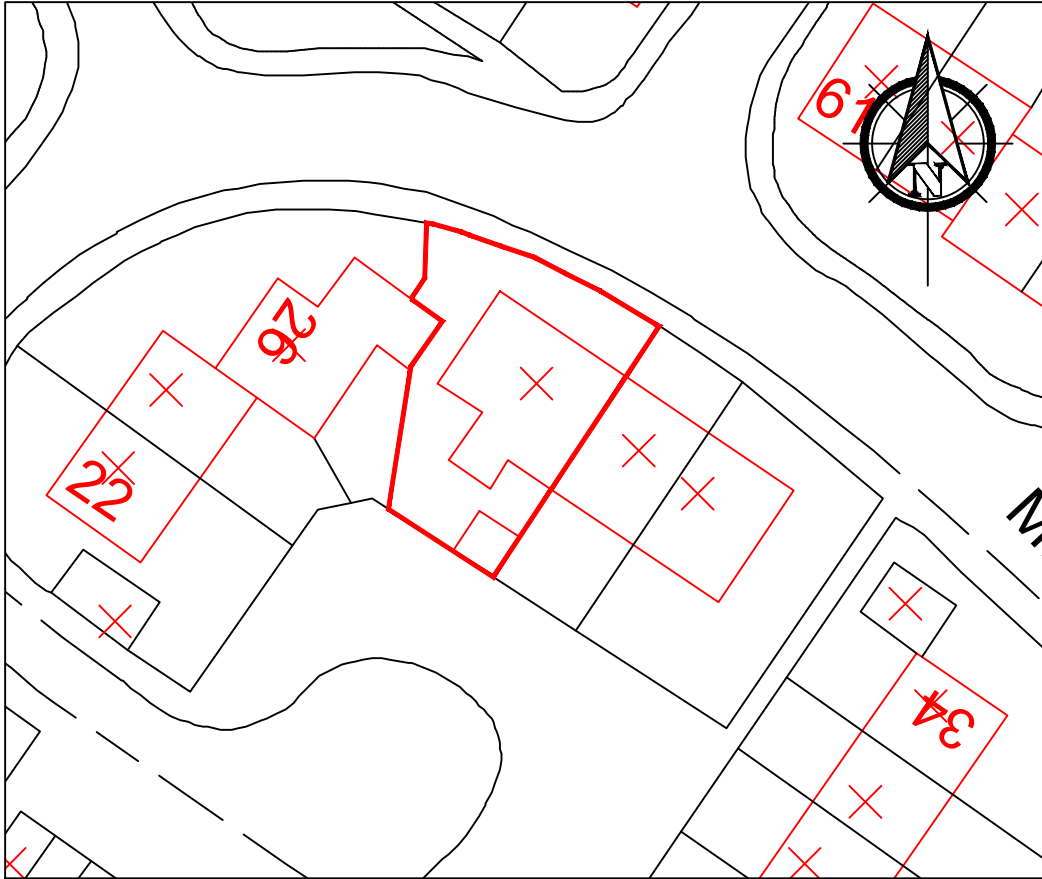
Block Plan 1/500
