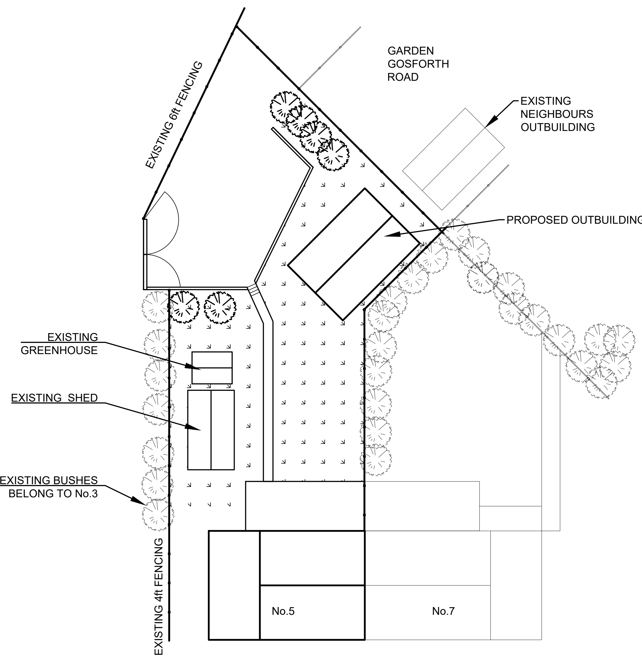
PROPOSED PLAN VIEW SCALE 1:50 PV1 Rev B
