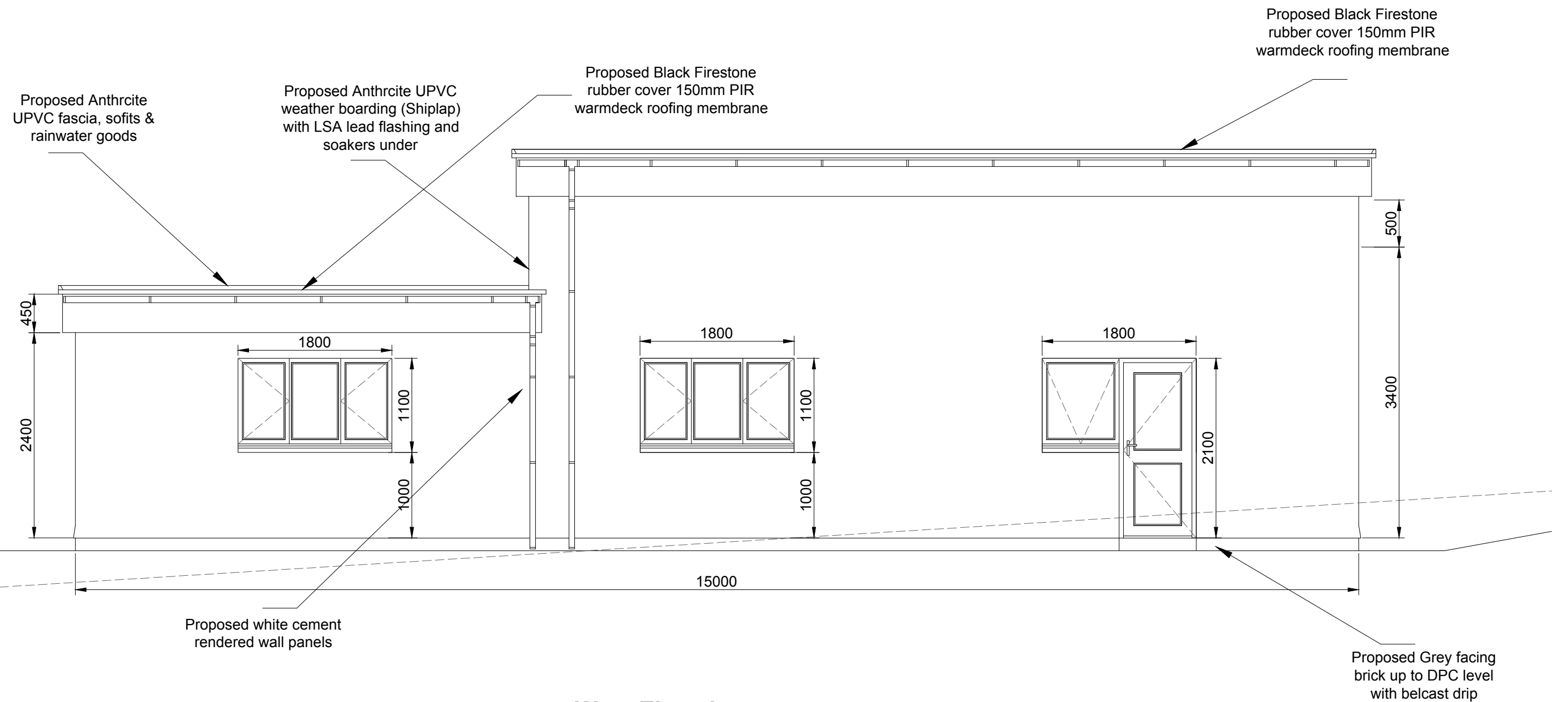
West Elevation
