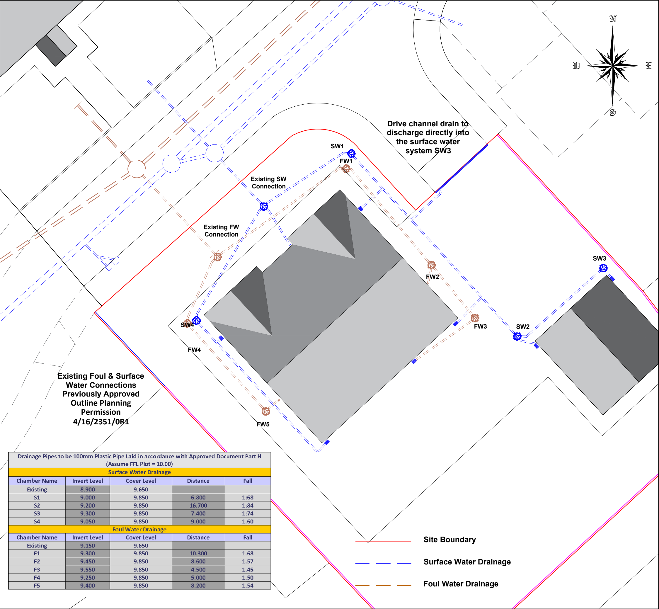
Proposed Drainage Plan 1/200
