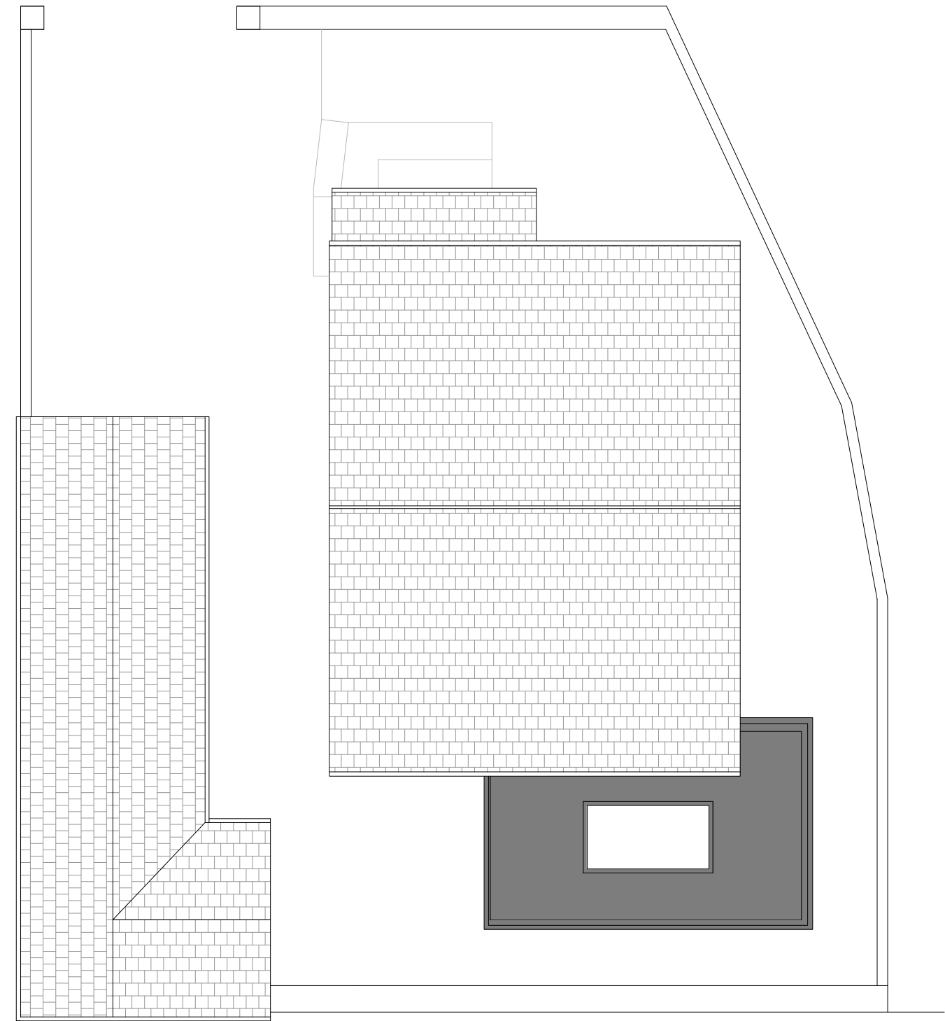
Proposed Roof Plan 1:100 @ A3
