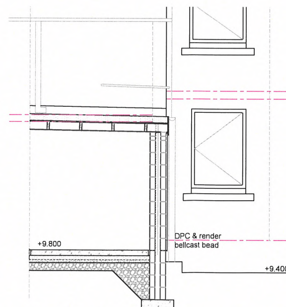
Section 1:50
