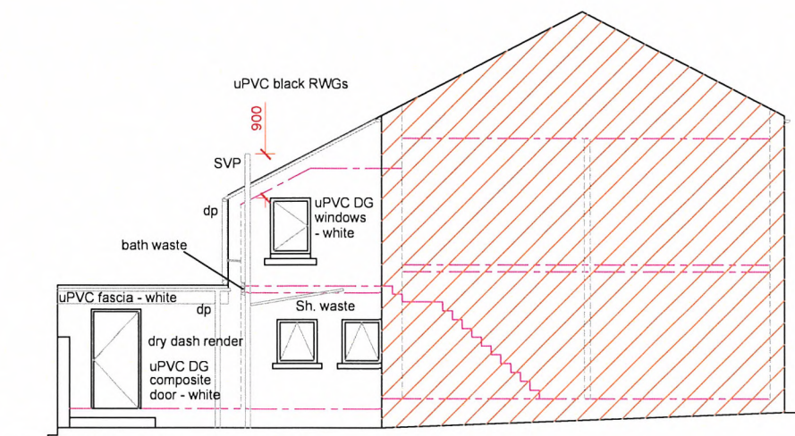
Side Elevation
