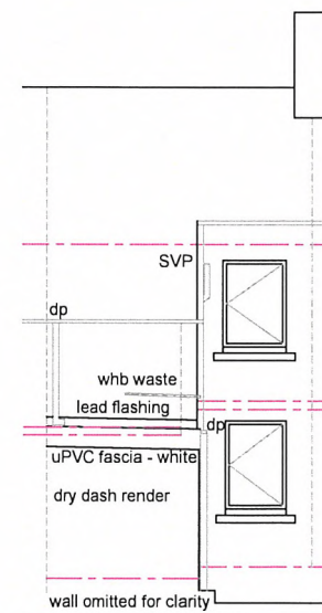
Rear Elevation
