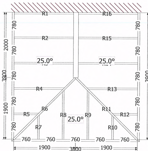
Roof Plan
