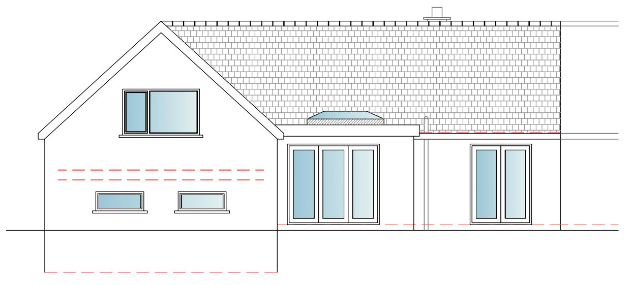
Rear Elevation
