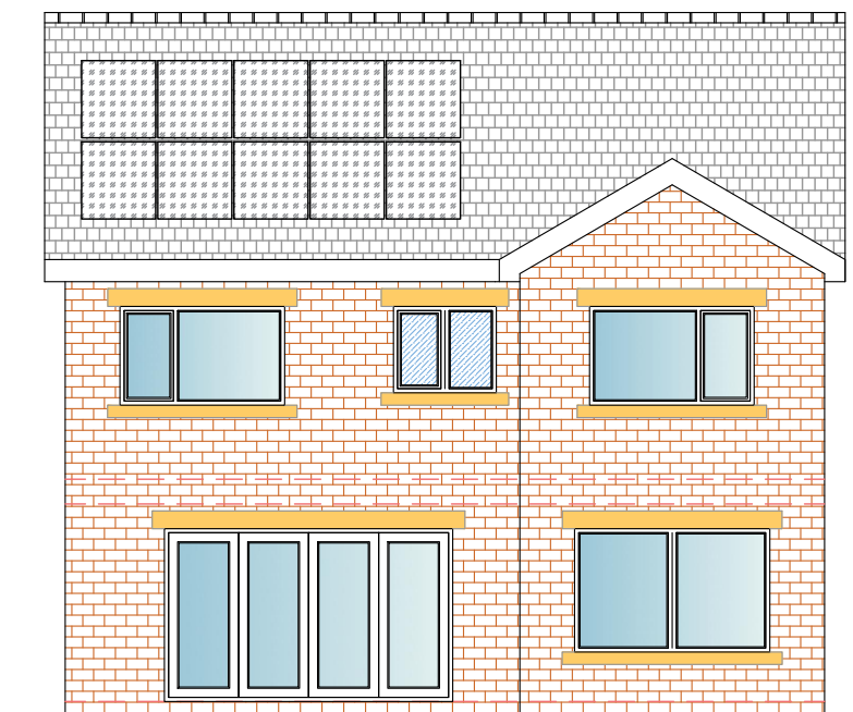
Rear Elevation
