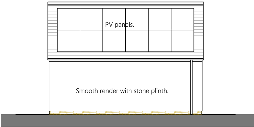
South-west Elevation
