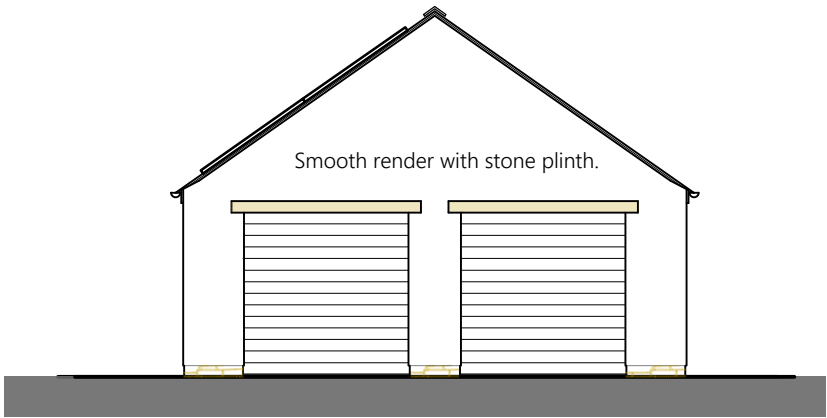
South-east Elevation
