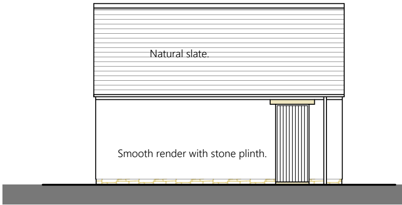
North-east Elevation
