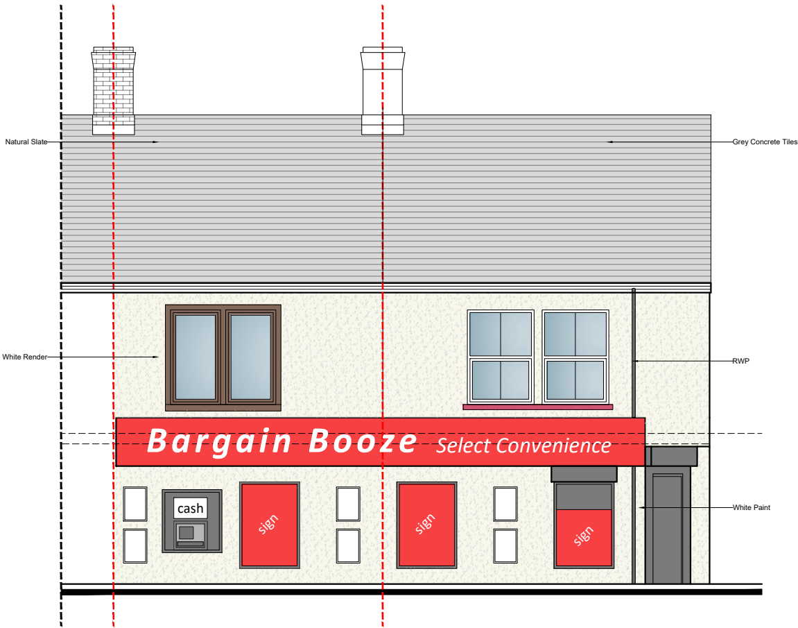
PROPOSED SOUTHERN ELEVATION Scale 1:100 @ A3
