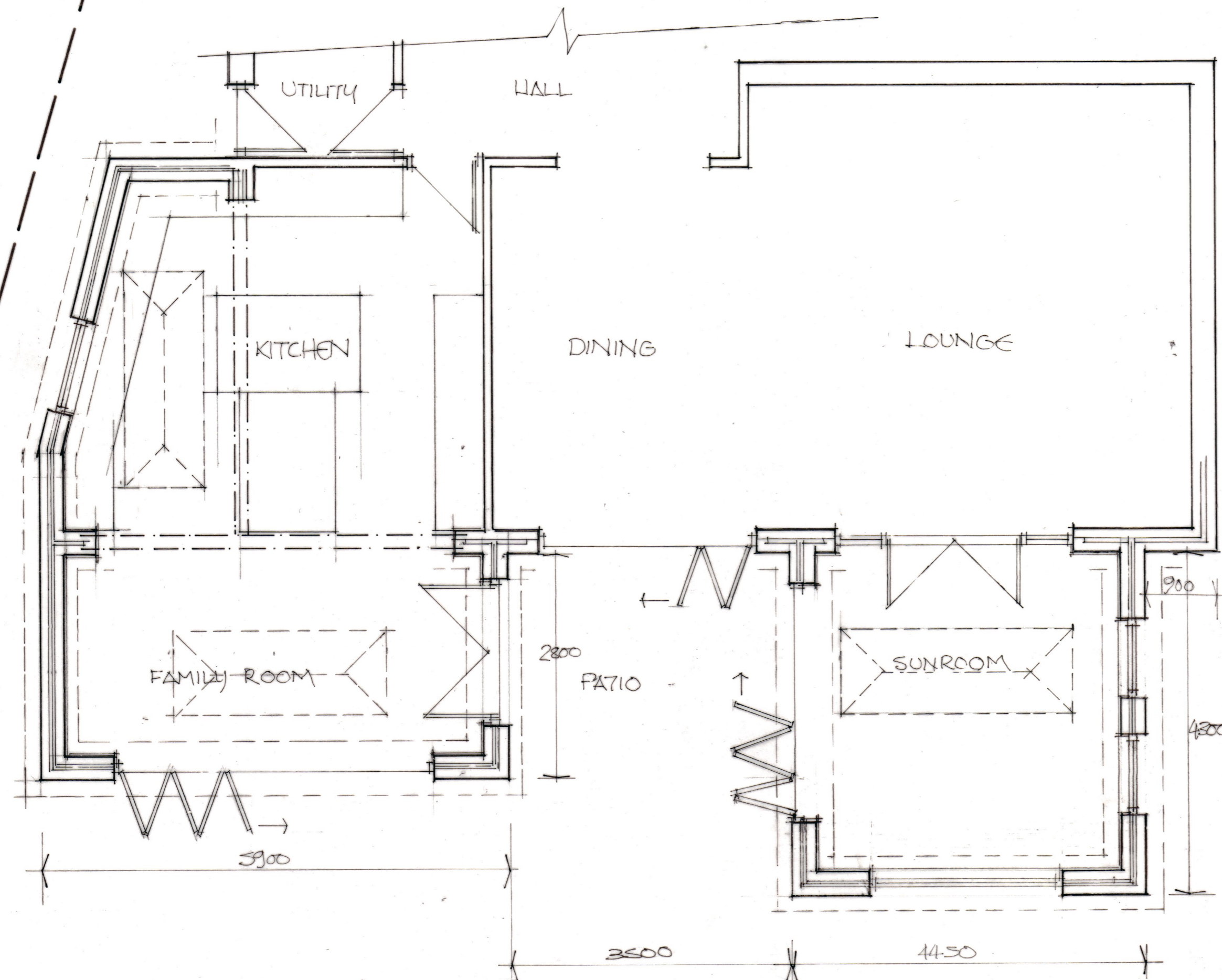
G.F. PLAN
