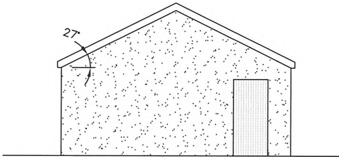
PROPOSED REAR ELEVATION SCALE 1:100 @ A3
