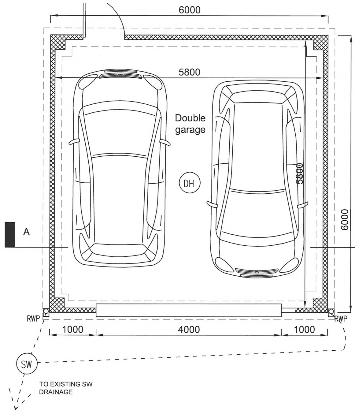
PROPOSED FLOOR PLAN SCALE 1:50 @ A3
