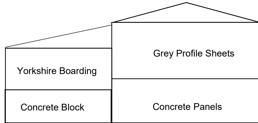
North Elevation
