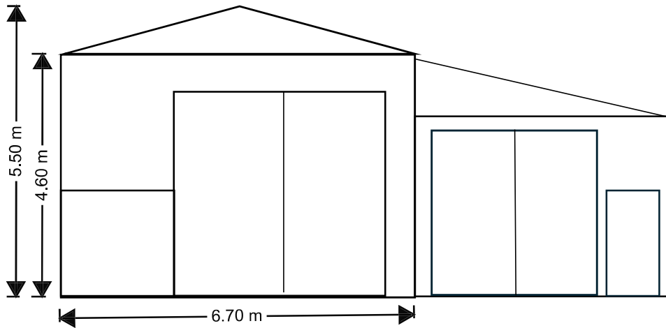
South Elevation
