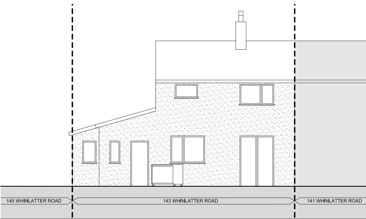
PROPOSED REAR ELEVATION (WEST) 1:100
