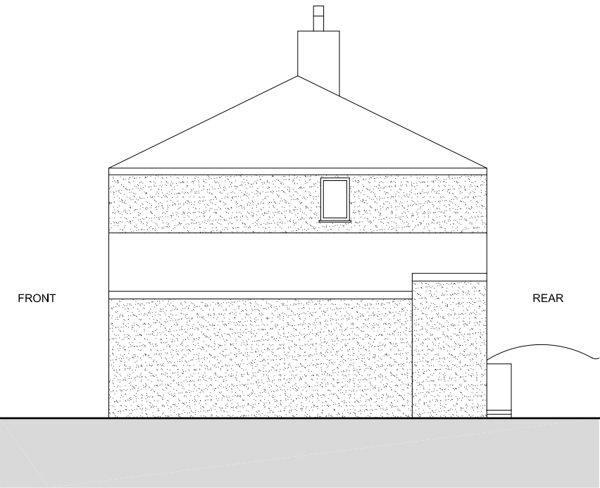
PROPOSED SIDE ELEVATION (NORTH) 1:100
