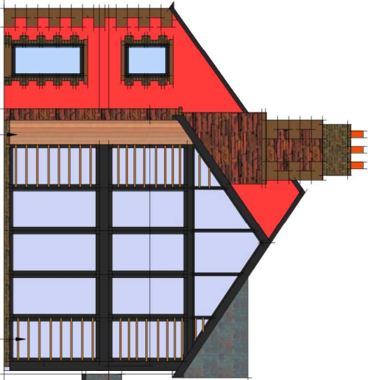
PROPOSED REAR
