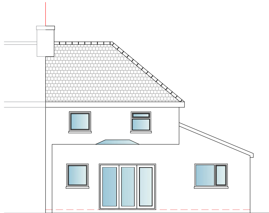
Rear Elevation
